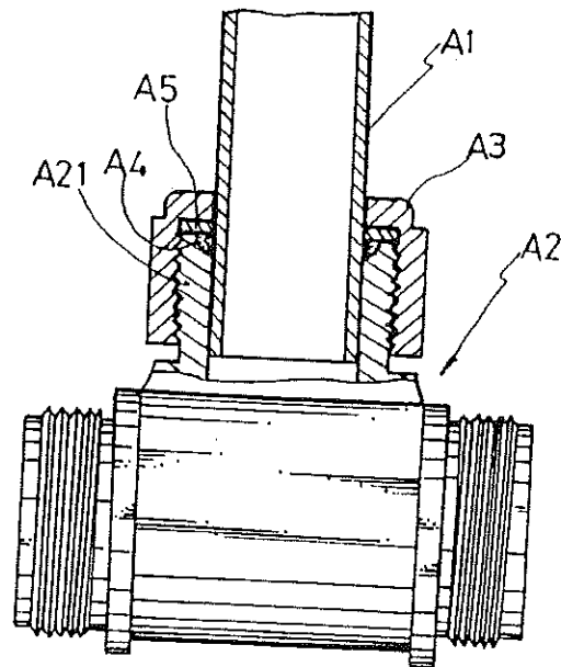
FIG.7 PRIOR ART
