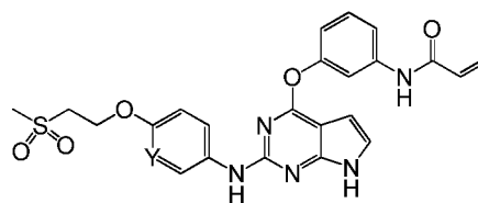
I-31 (Y = CH, CF, N)
