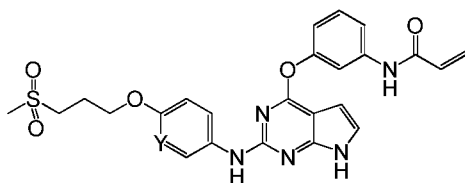
I-32 (Y = CH, CF, N)
