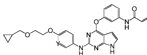
I-35 (Y = CH, CF, N)
