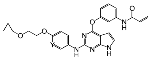
I-40 (Y = CH, CF, N)
