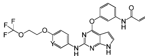
I-33 (Y = CH, CF, N)
