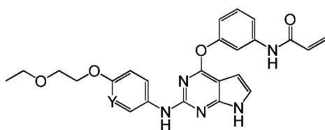
I-34 (Y = CH, CF, N)
