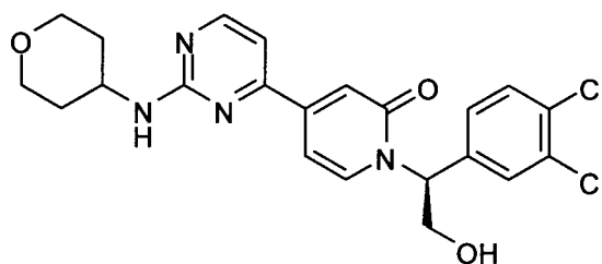
( S )-1-(1-(3,4-dichlorophenyl)-2-hydroxyethyl)-4-(2-((tetrahydro-2 H -pyran-4-yl)amino)pyrimidin-4-yl)pyridin-2(1 H )-one
