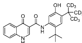
deuterated ivacaftor
