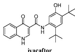
ivacaftor
