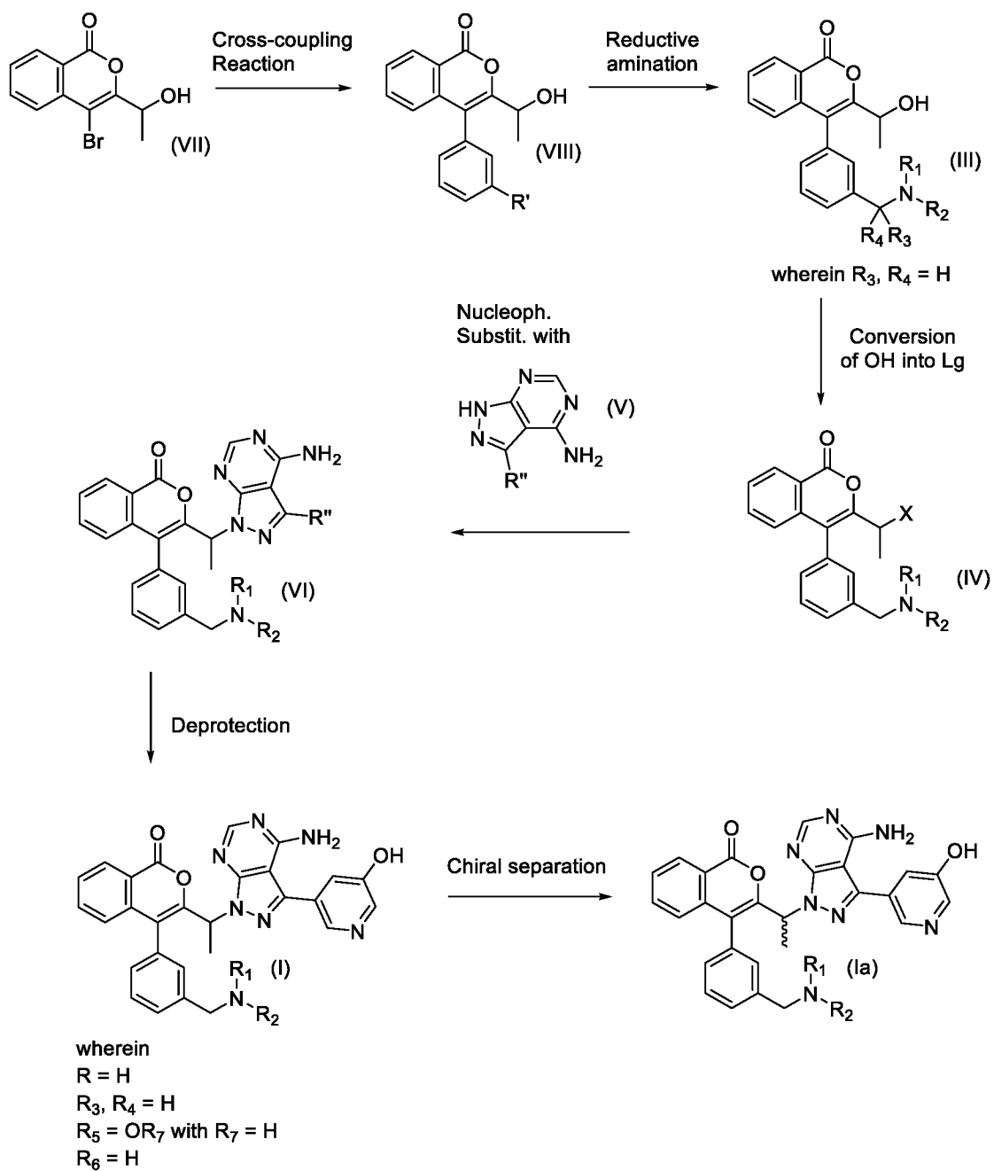
Scheme 1
