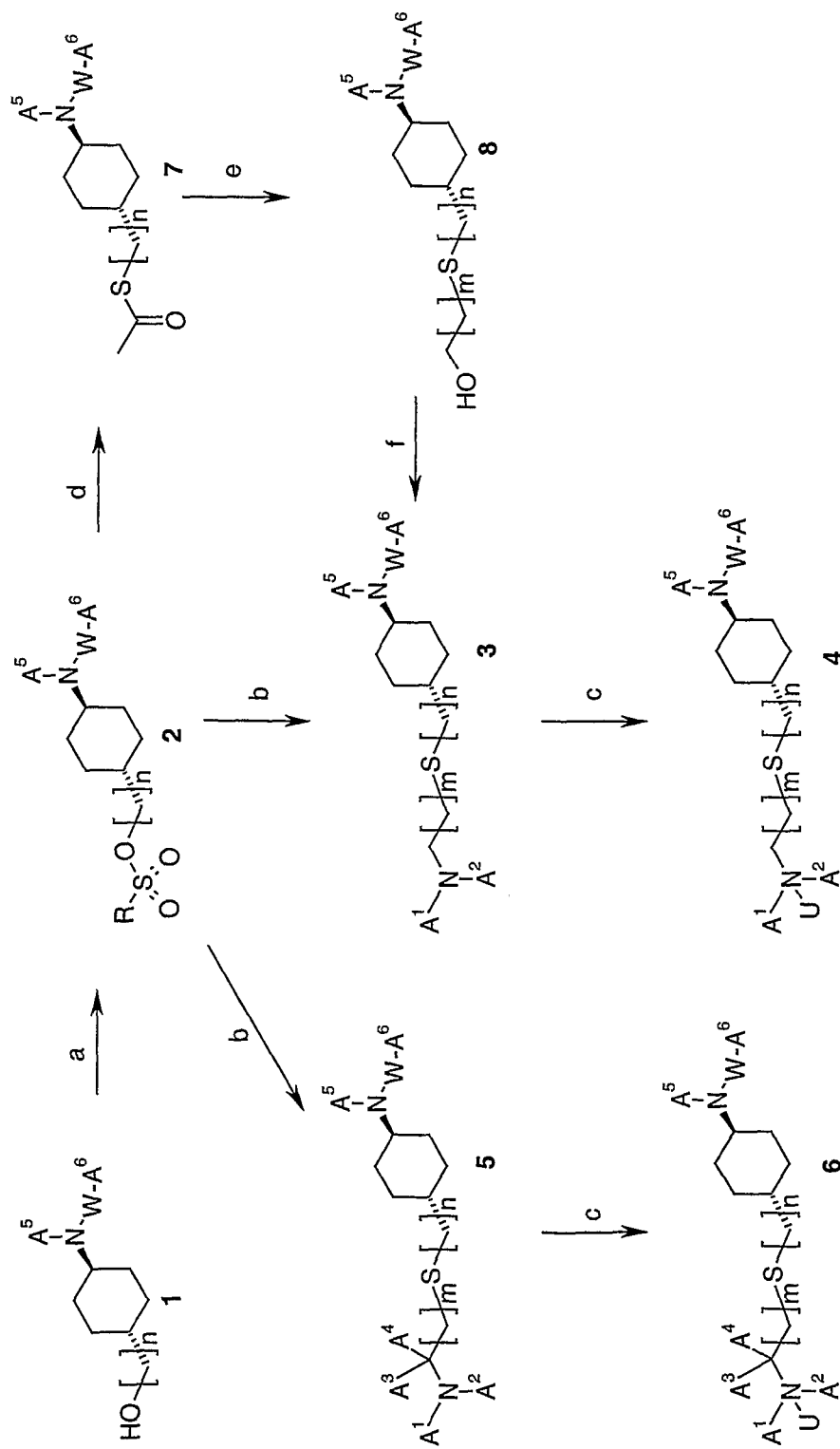
Scheme 4
