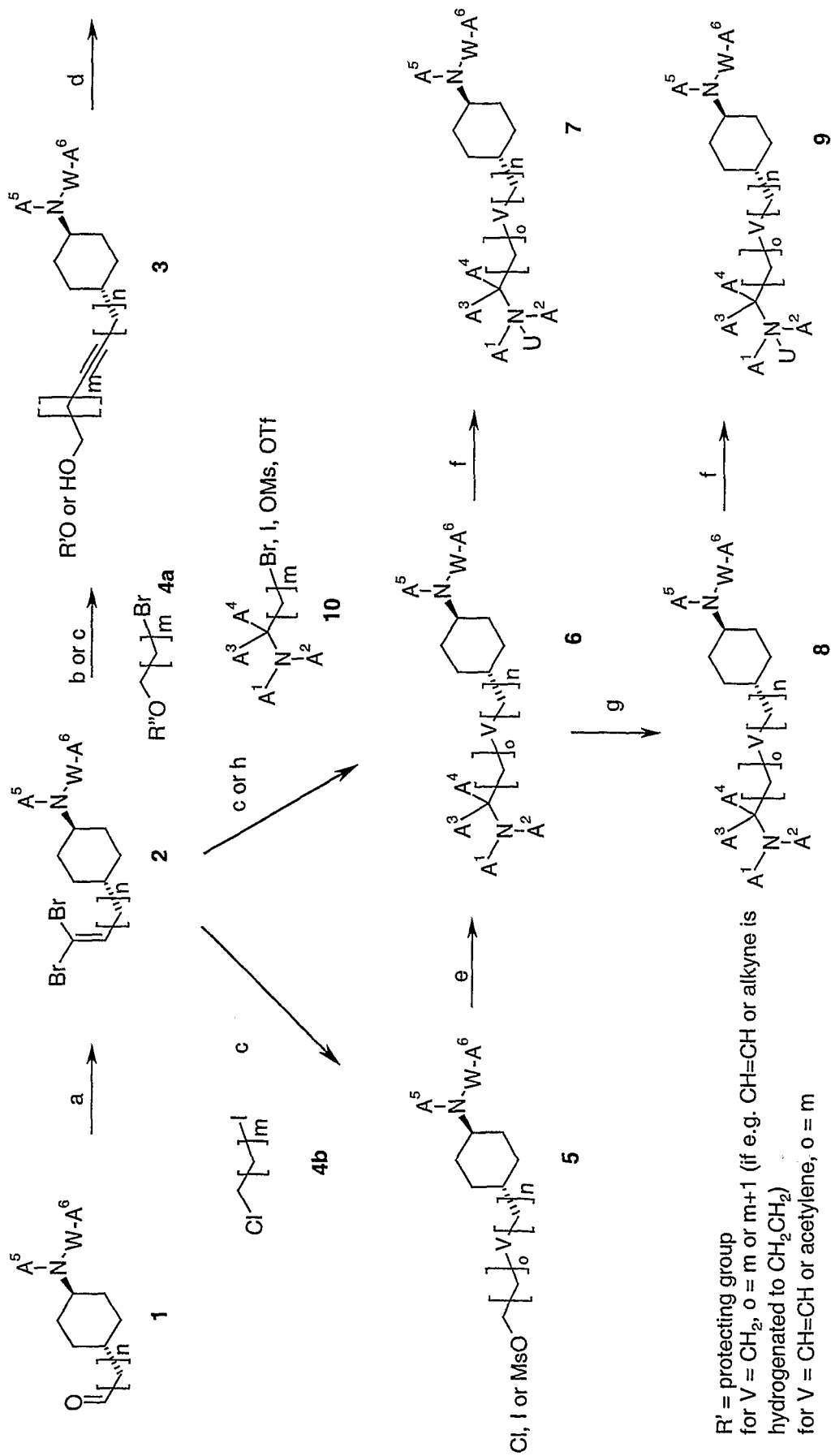
Scheme 5
