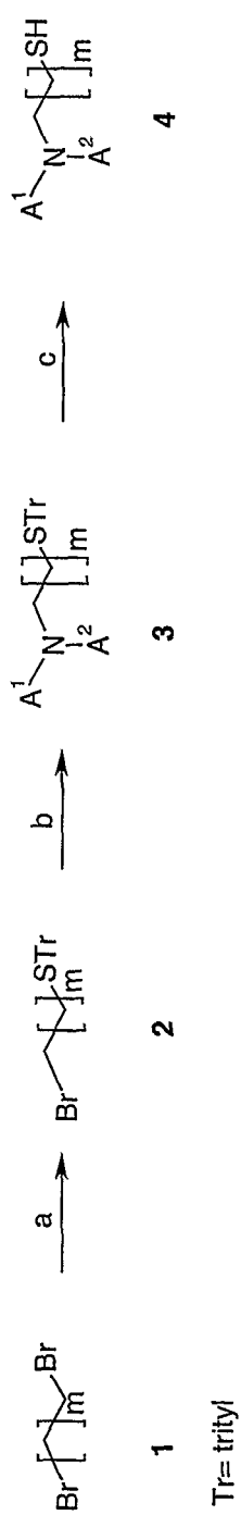
Scheme 2
