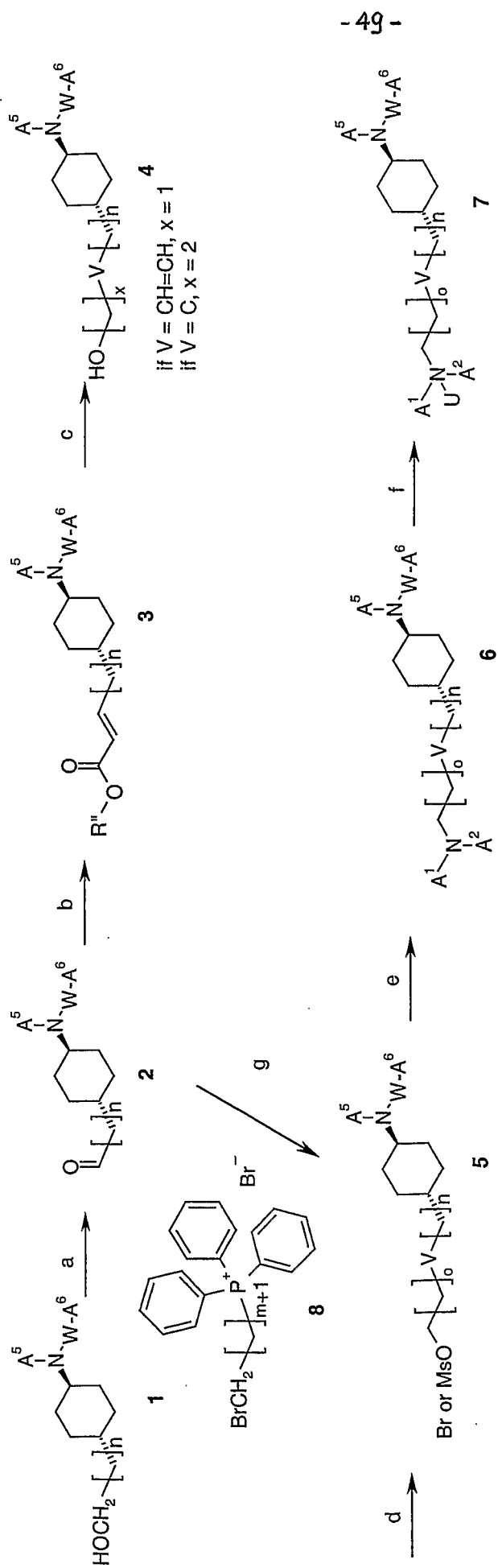
Scheme 6
