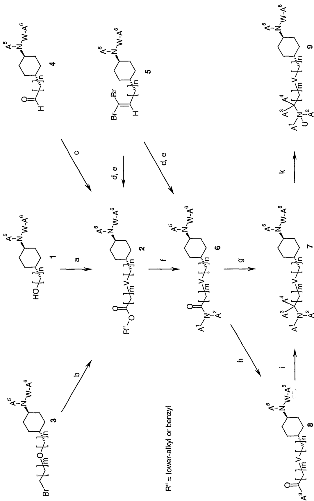
Scheme 7
