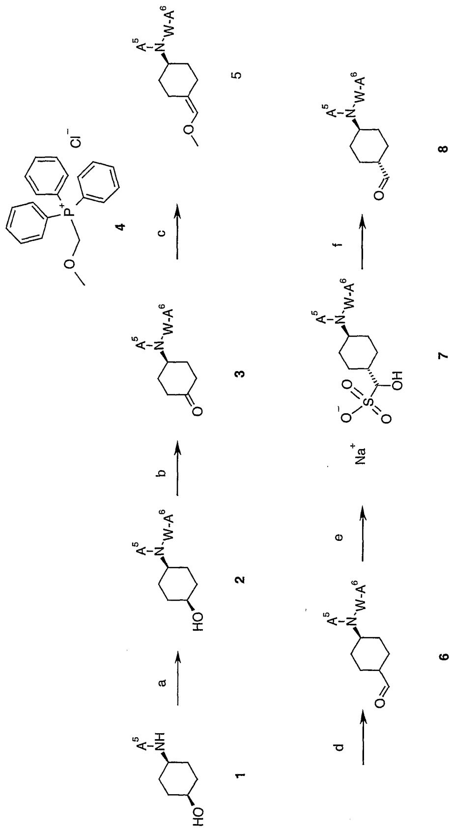
Scheme 1b
