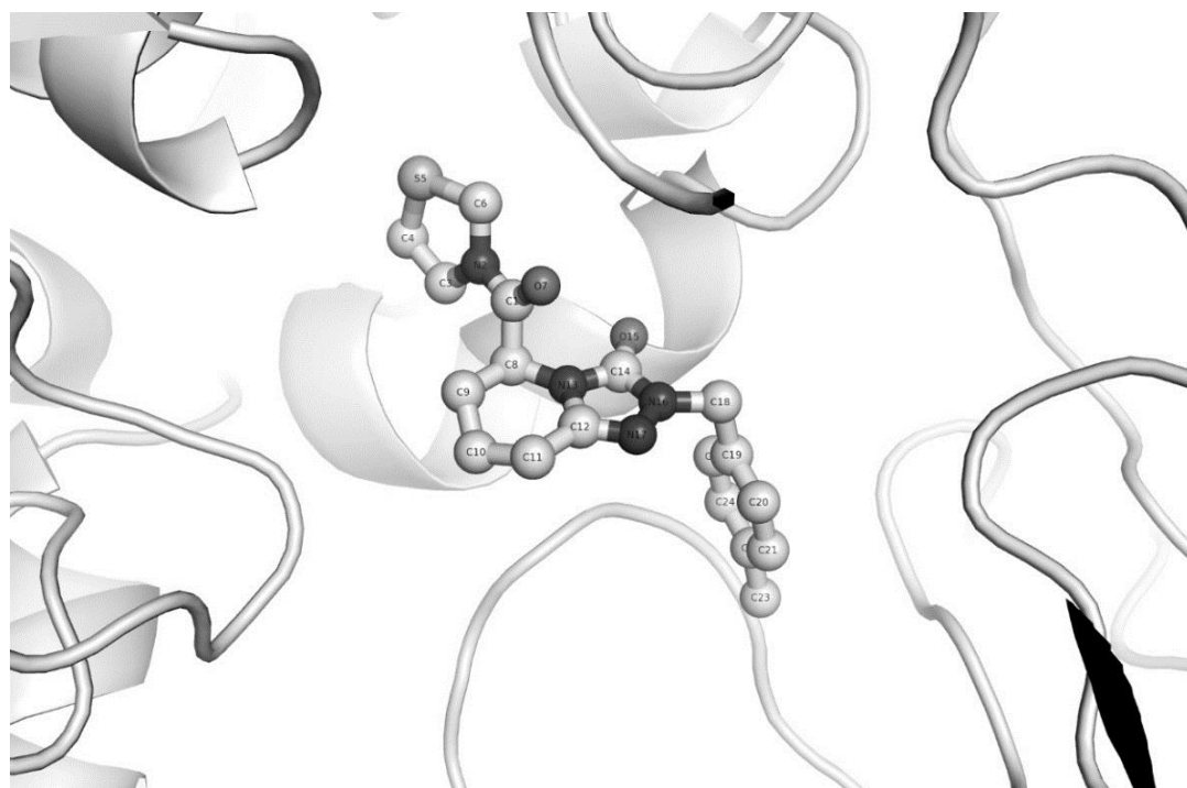
Figure 4, Example 108 in a complex with PREP (porcine)
