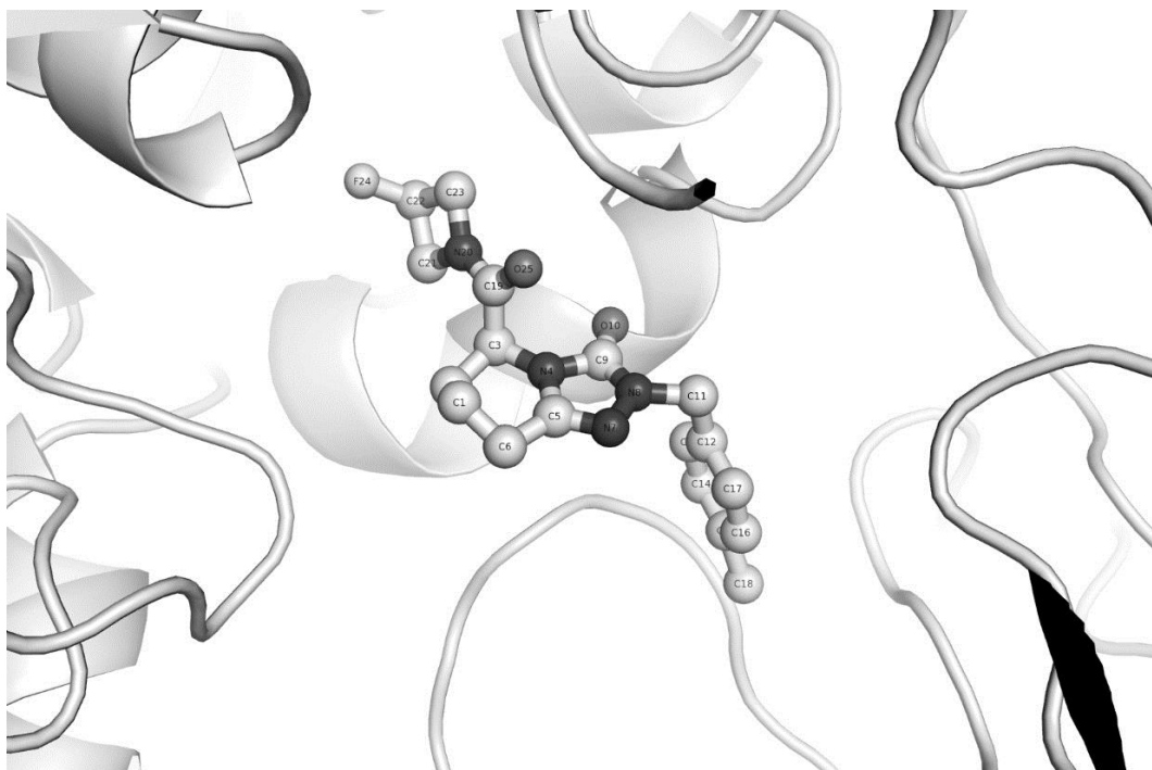
Figure 5, Example 113 in a complex with PREP (porcine)
