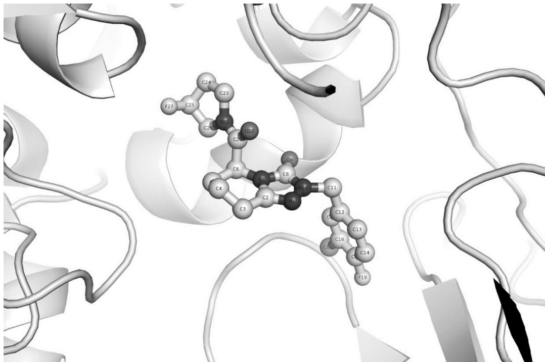
Figure 3, Example 454 in a complex with PREP (porcine)
