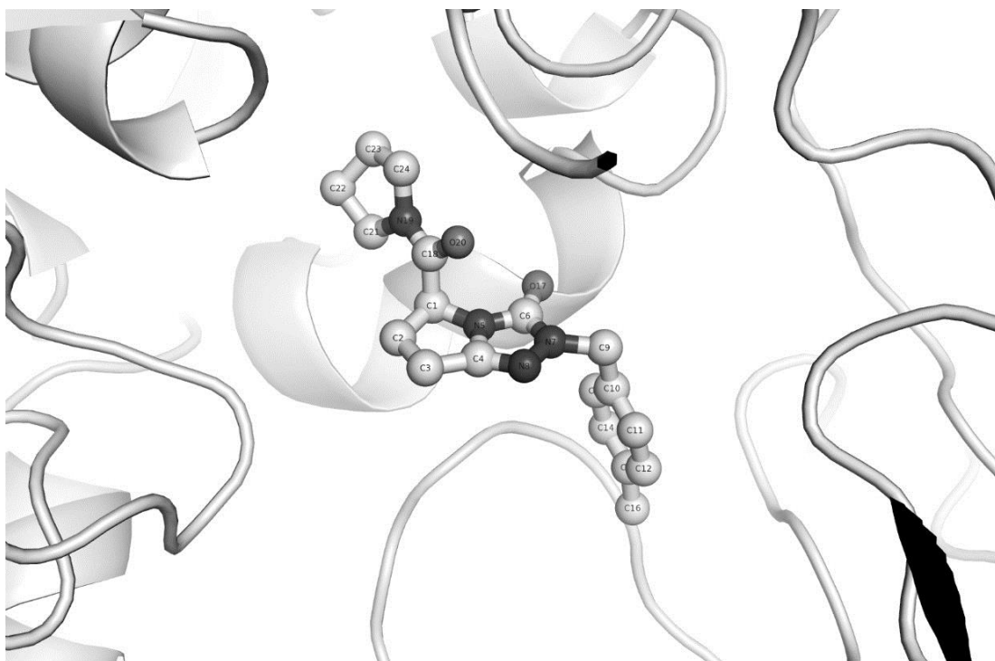
Figure 6, Example 157 in a complex with PREP (porcine)
