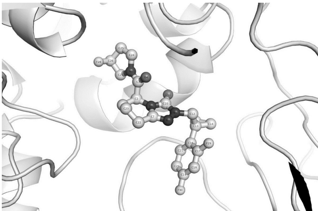
Figure 2, Example 358 in a complex with PREP (porcine)
