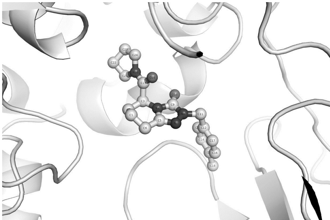
Figure 7, Example 26 in a complex with PREP (porcine)
