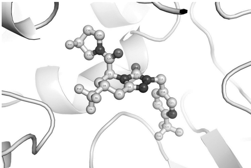
Figure 1, Example 237 in a complex with PREP (porcine)
