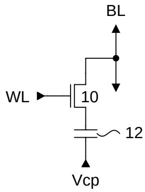
FIG. 1 (Prior Art)
