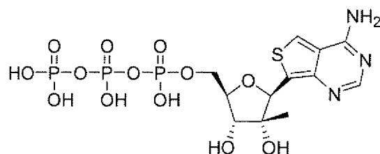
Compound 4
