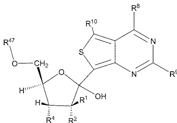
Formula IX
