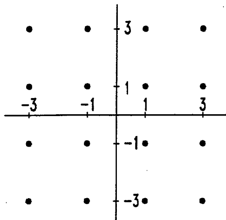
STANDARD 16-QAM
