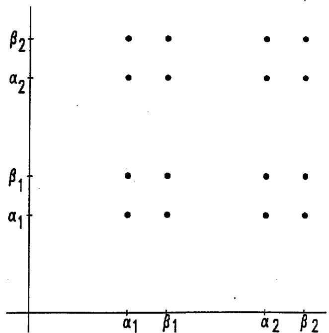
(2,2,2;6) C-R MAPPED 64-QAM
