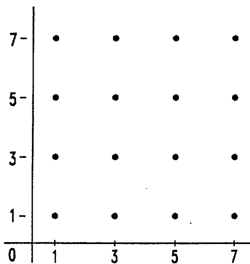
STANDARD 64-QAM
