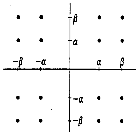
(2,2;4) C-R MAPPED 16-QAM
