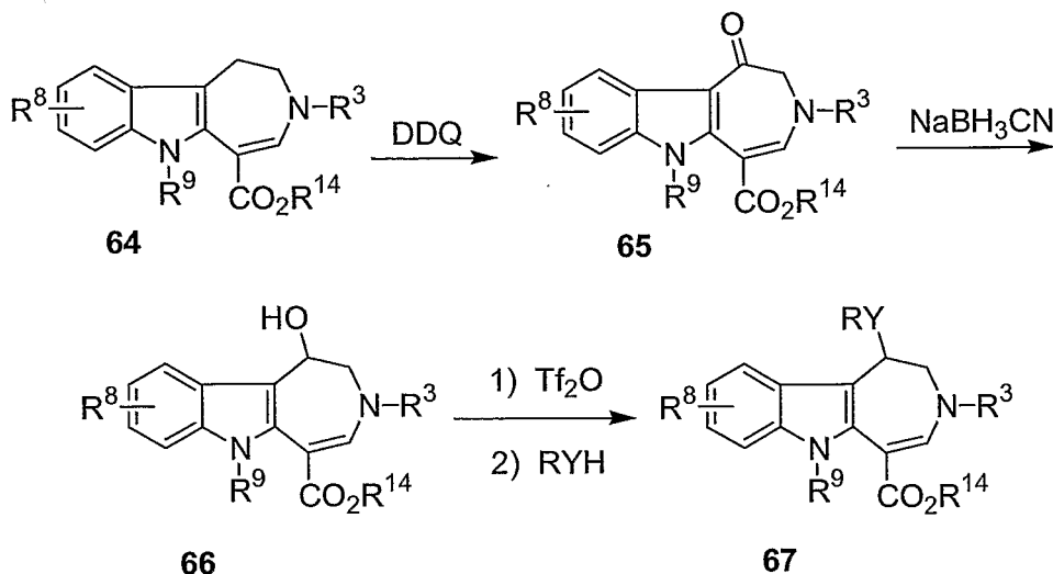
SCHEME 23
