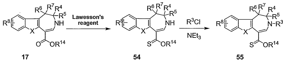
SCHEME 19
