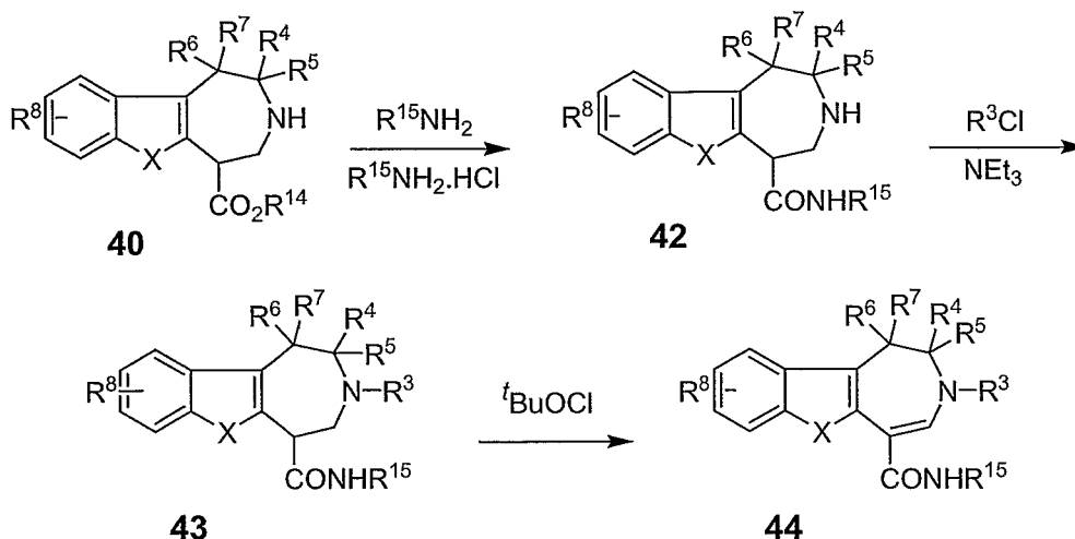
SCHEME 15
