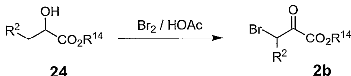
SCHEME 9
