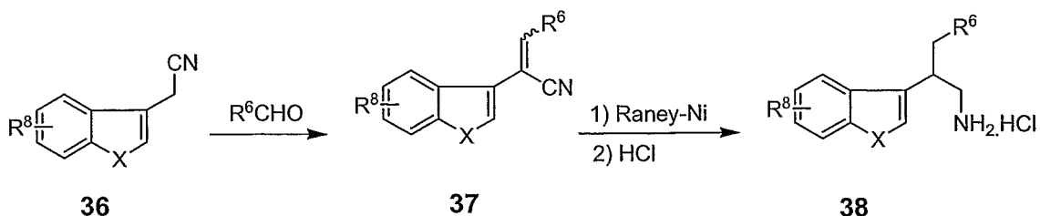
SCHEME 13
