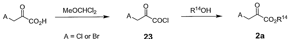
SCHEME 8
