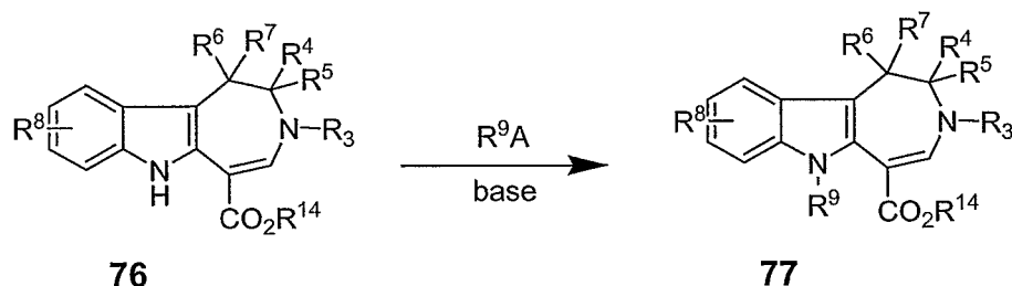
SCHEME 27
