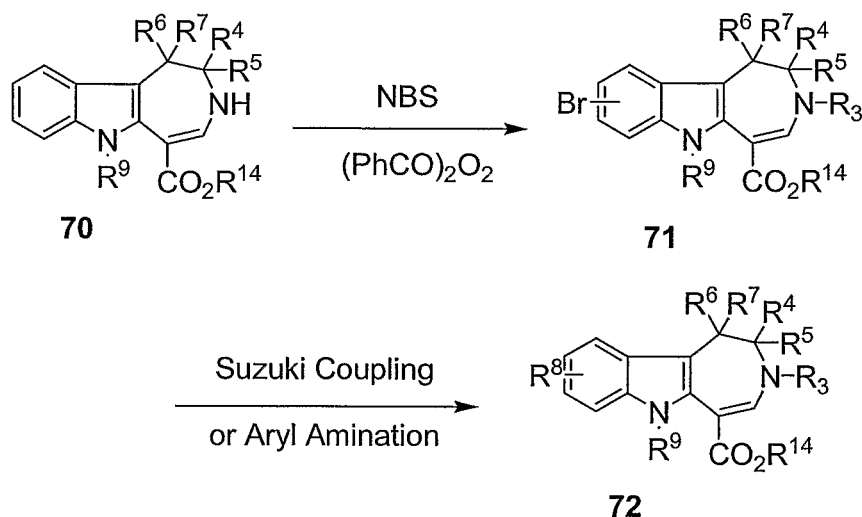
SCHEME 25
