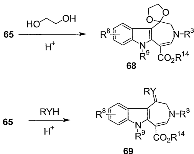
SCHEME 24
