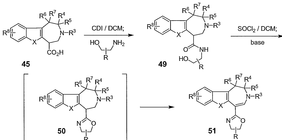
SCHEME 17
