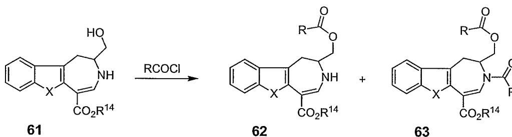
SCHEME 22
