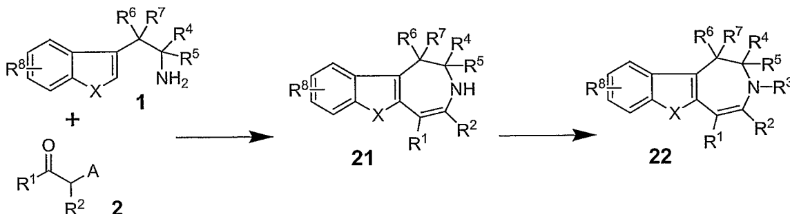
SCHEME 7
