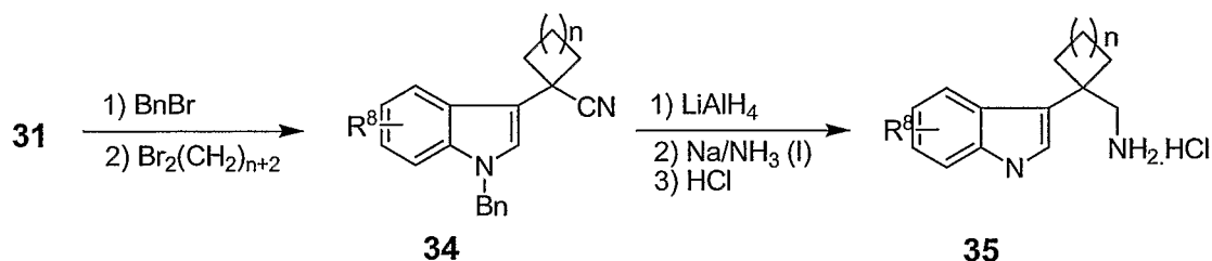
SCHEME 12
