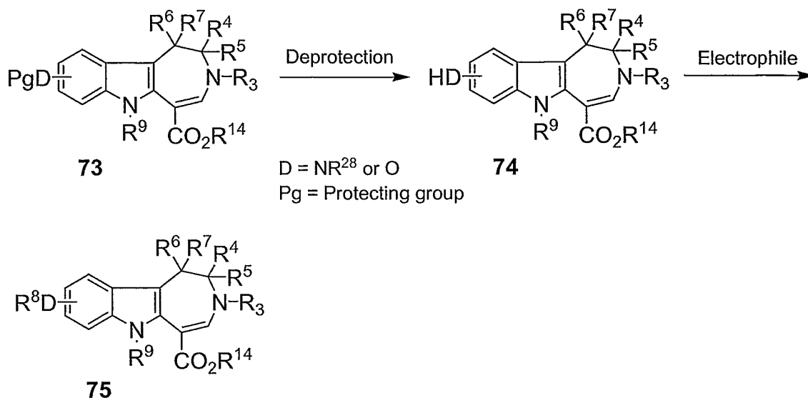
SCHEME 26
