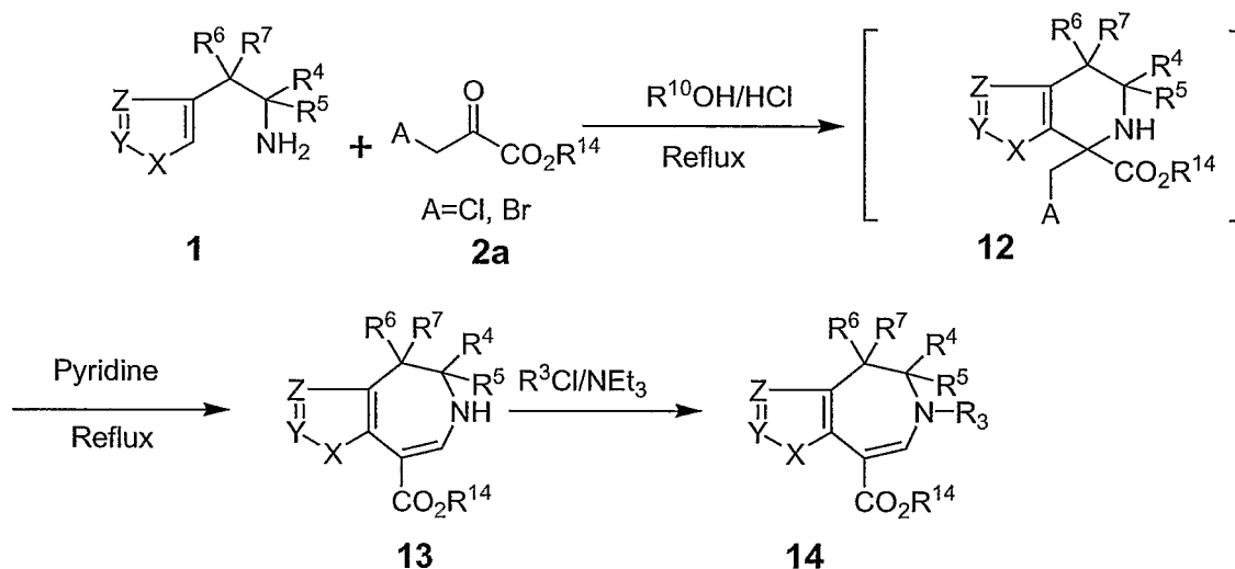
SCHEME 4
