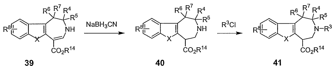
SCHEME 14
