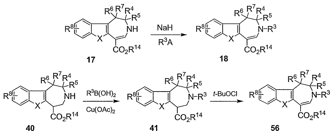
SCHEME 20
