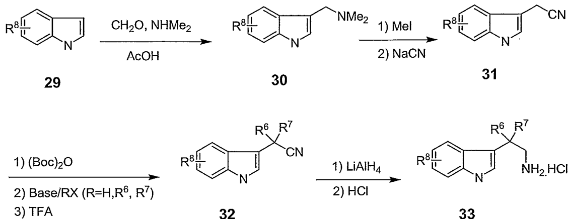
SCHEME 11
