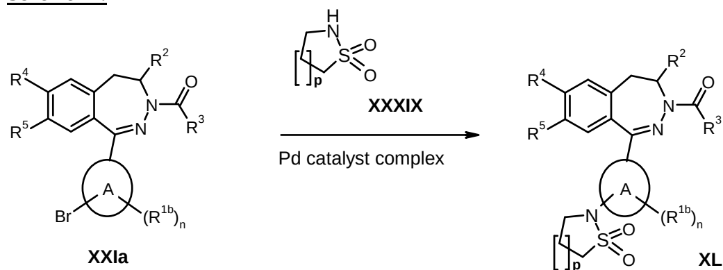
Scheme 11:
