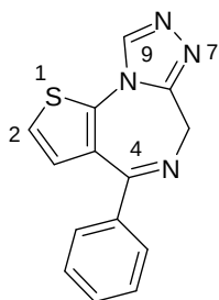
4-Phenyl-6H-thieno[3,2-f][1,2,4]triazolo[4,3-a][1,4]diazepine
