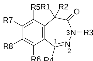
substituted 3,5-Dihydro-4H-2,3-benzodiazepine-4-ones
