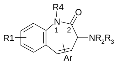
substituted 3-Amino-2,3-dihydro-1H-1-benzazepine-2-ones
