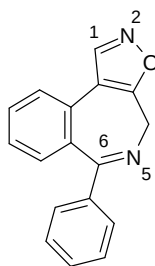
6-Phenyl-4H-isoxazolo[5,4-d][2]benzazepine
