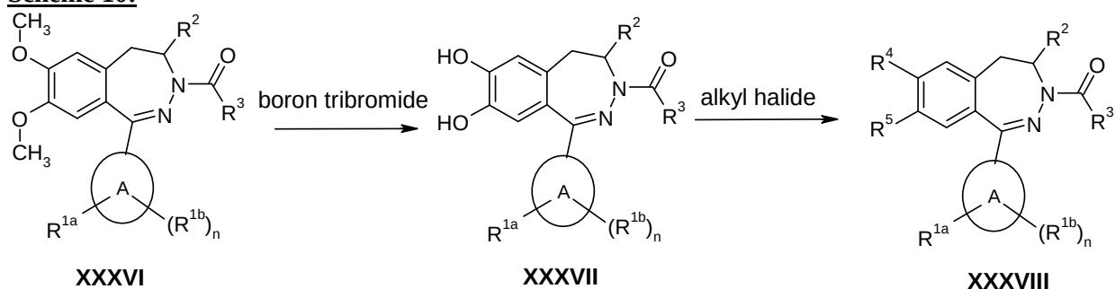
Scheme 10:
