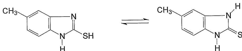
2-mercapto-5-methylbenzimidazole
