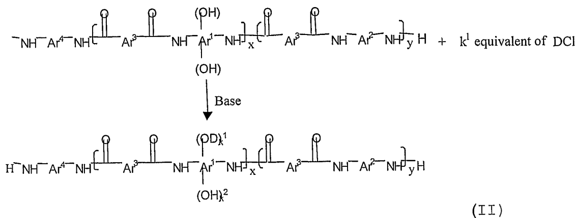
Reaction 1
