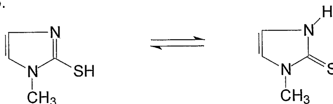
2-mercapto-1-methylimidazole
