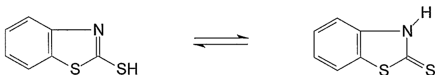
2-mercaptobenzothiazole
