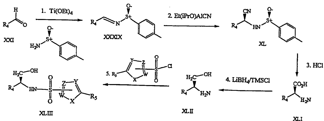
Scheme 11
