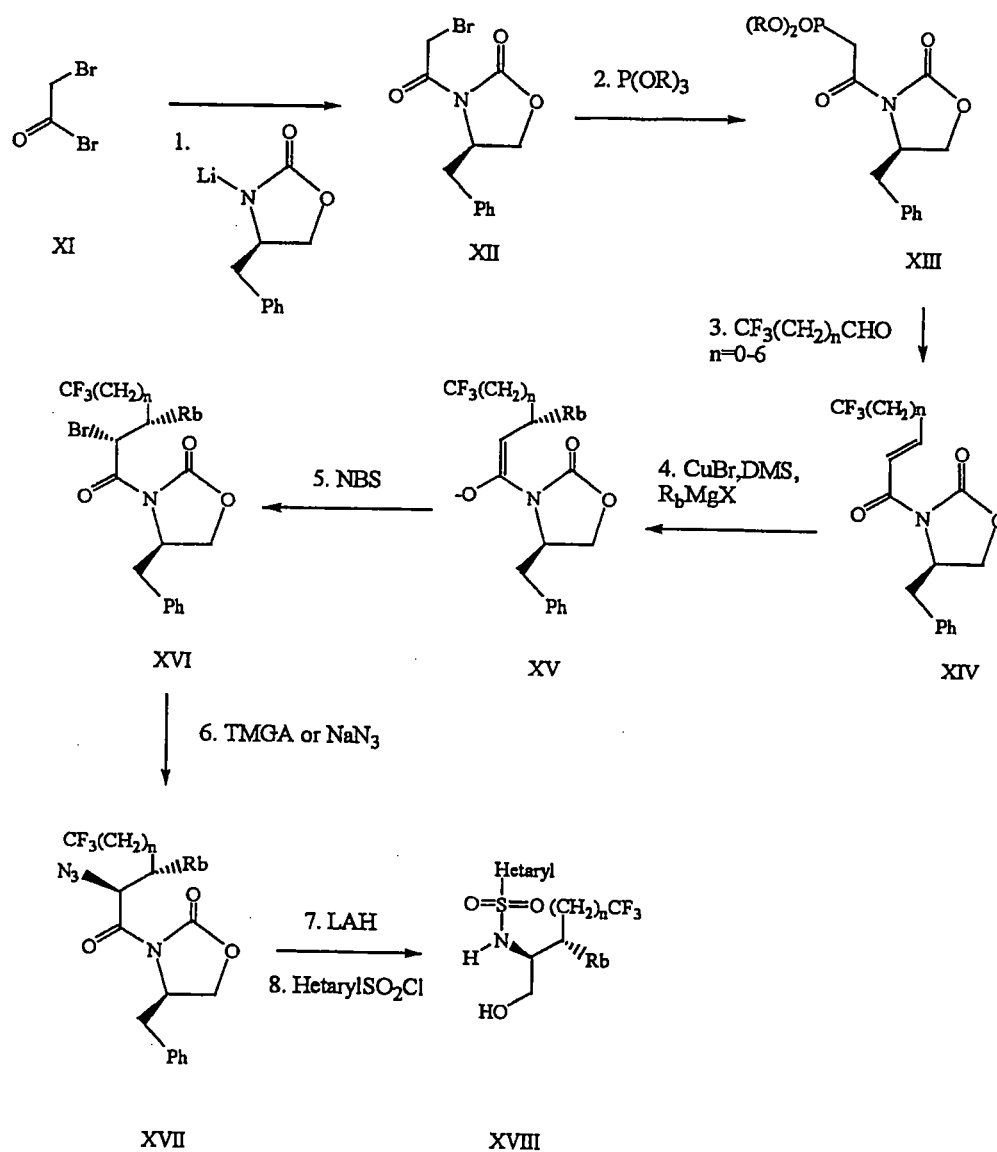
Scheme 4
