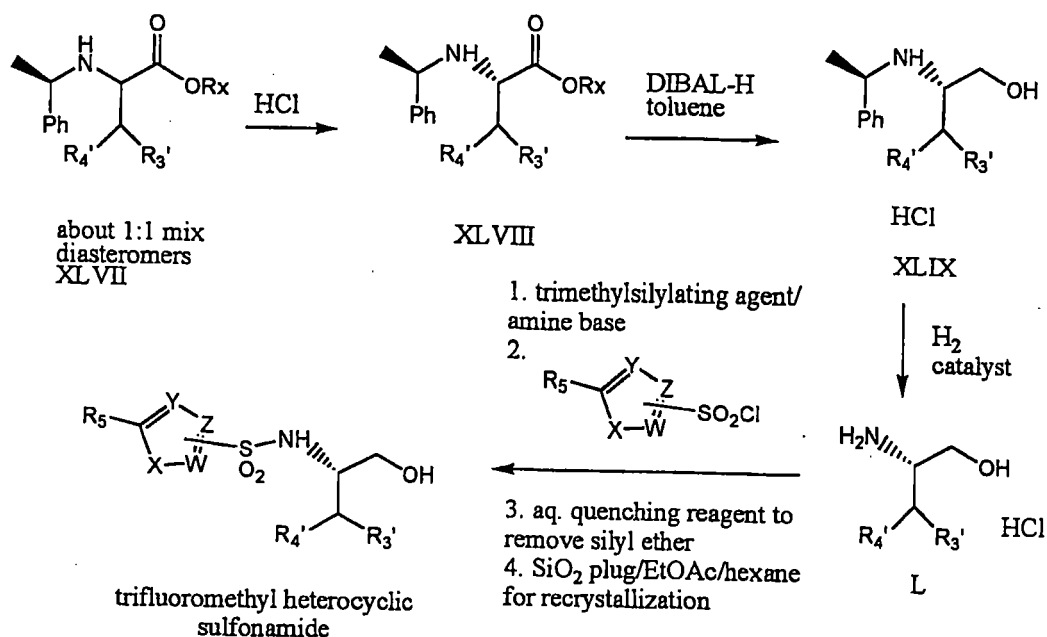
Scheme 13
