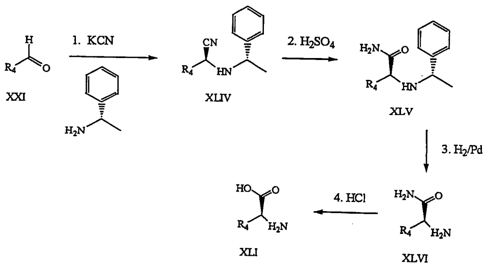
Scheme 11
