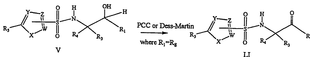
Scheme 14
