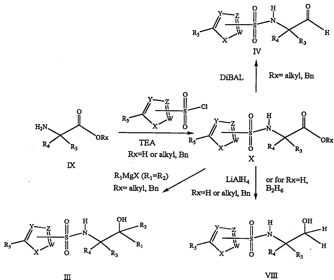
Scheme 2
