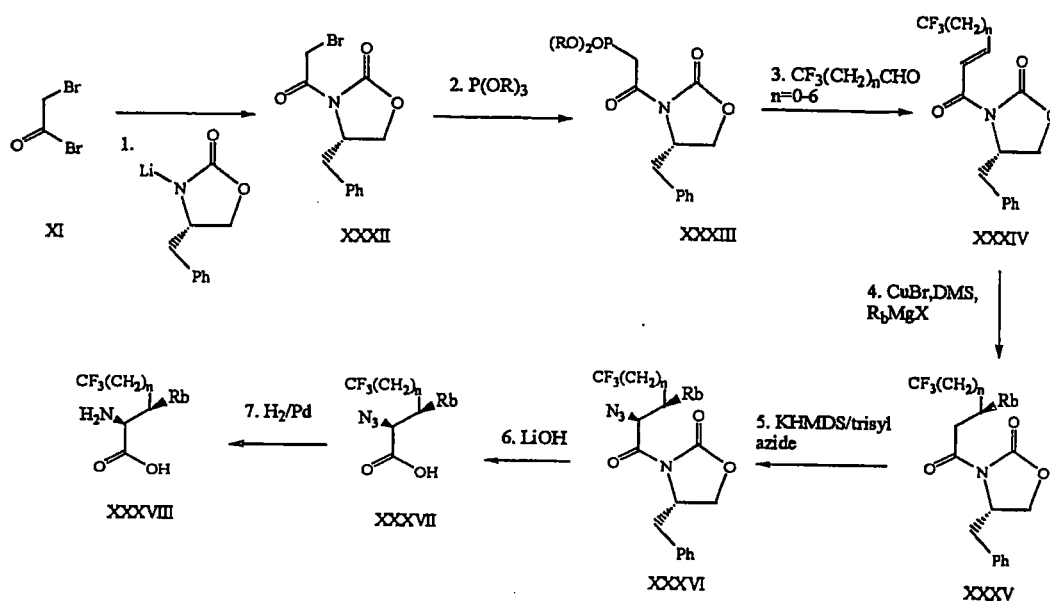
Scheme 9
