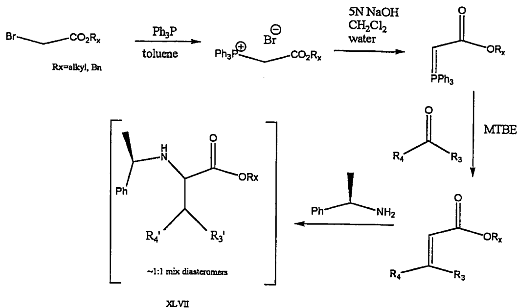
Scheme 12
