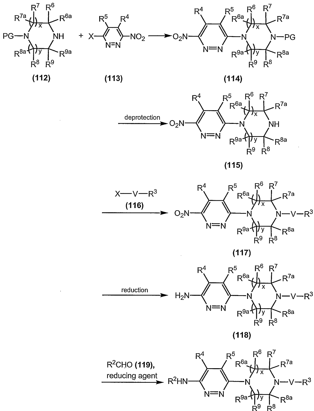
Formula (I)
