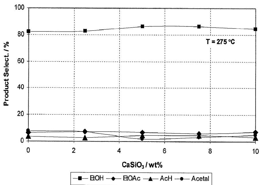
FIG. 6D - Selectivity @ 275
