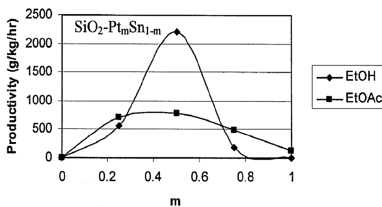
FIG. 1B - Productivity of Pt/Sn Catalyst
