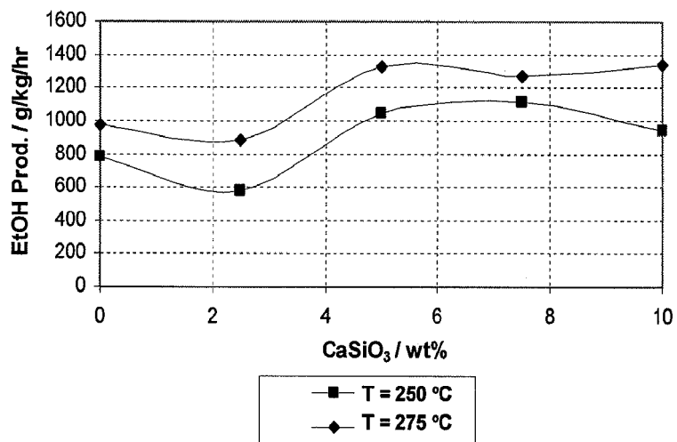
FIG. 6B - Productivity
