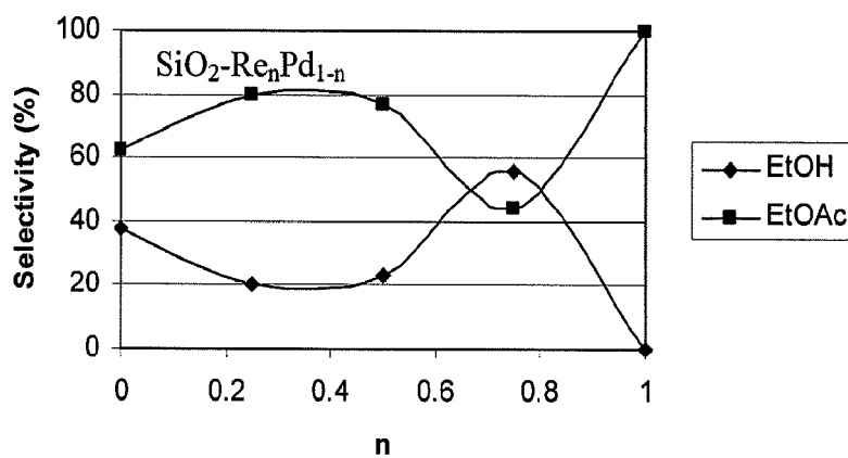
FIG. 2A - Selectivity of Re/Pd
