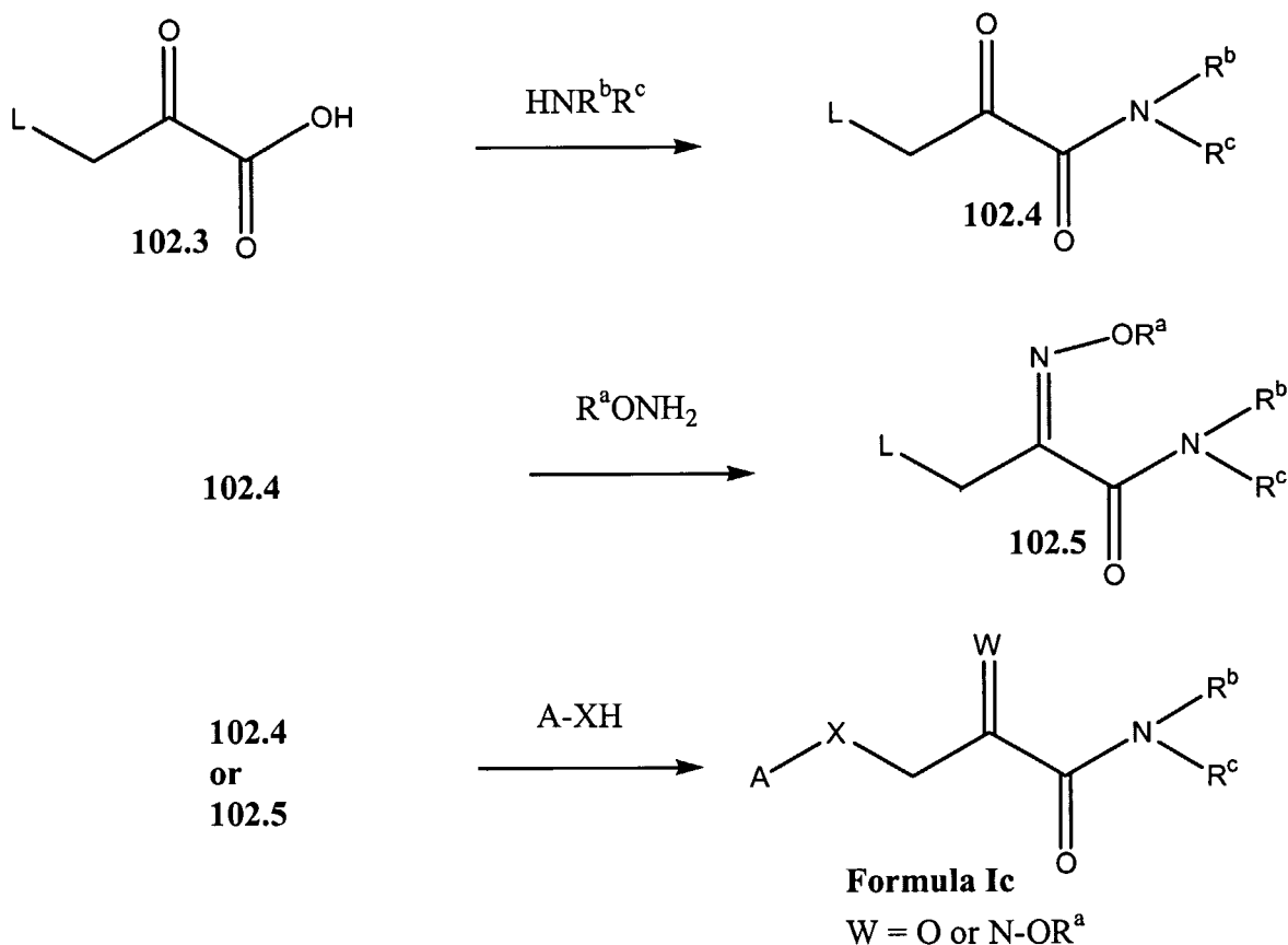
Reaction Scheme 1c
