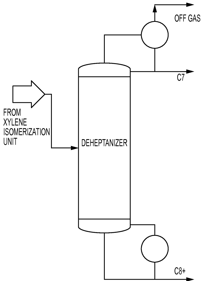
FIG. 2 PRIOR ART
