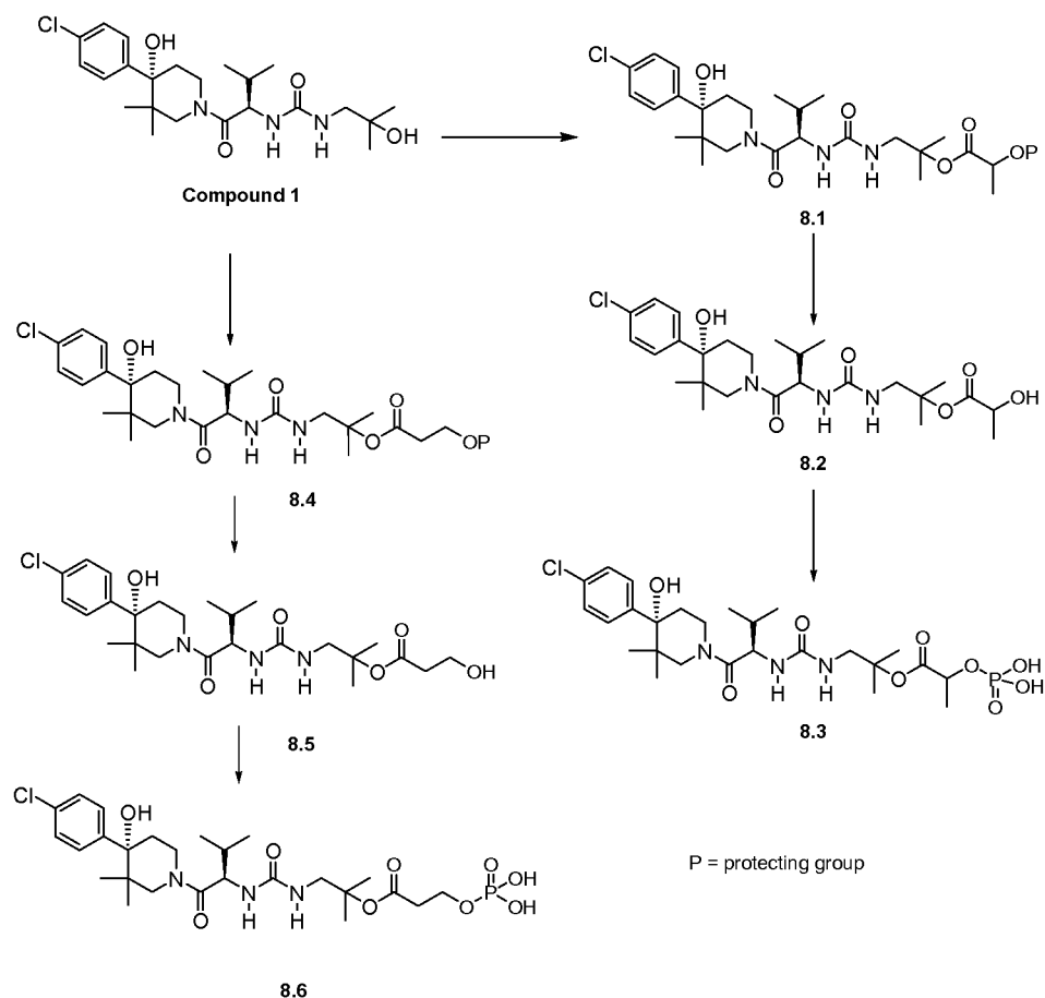
Scheme 8
