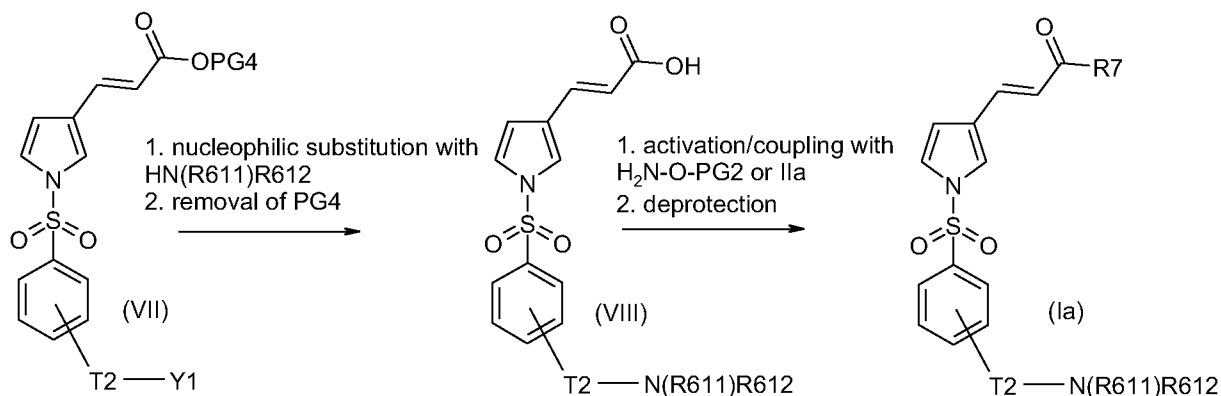
Reaction scheme 2:
