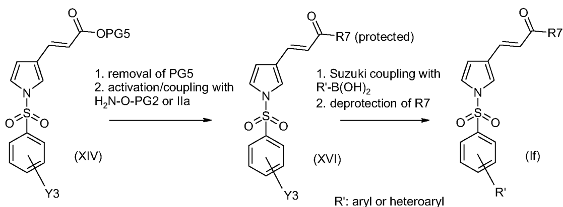
Reaction scheme 7:
