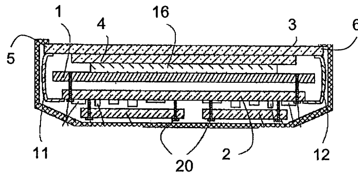
Fig.1 – PRIOR ART
