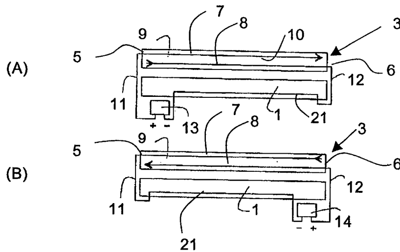
Fig.2 – PRIOR ART
