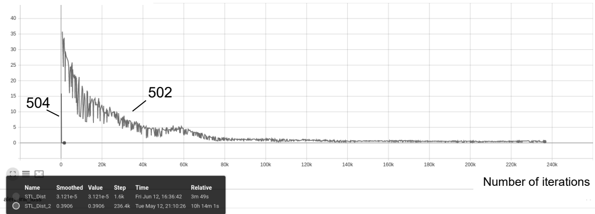
Autoencoder loss
