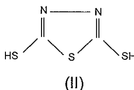
2,5-dimercapto-1,3,4-thiadiazole
