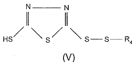
2-mercapto-5-hydrocarbyldithio-1,3,4-thiadiazole
