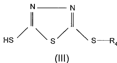
2-mercapto-5-hydrocarbylthio-1,3,4-thiadiazole
