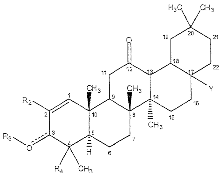
(XIII),
