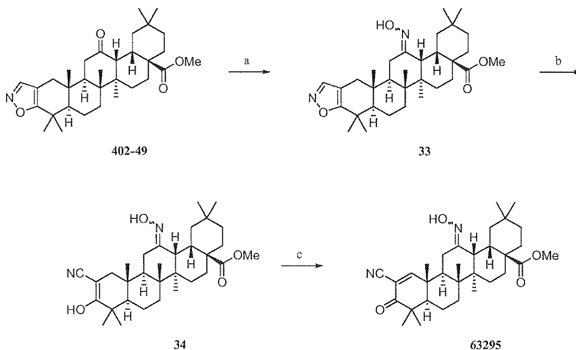
Scheme 16:
