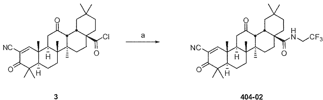
10 Scheme 4:
