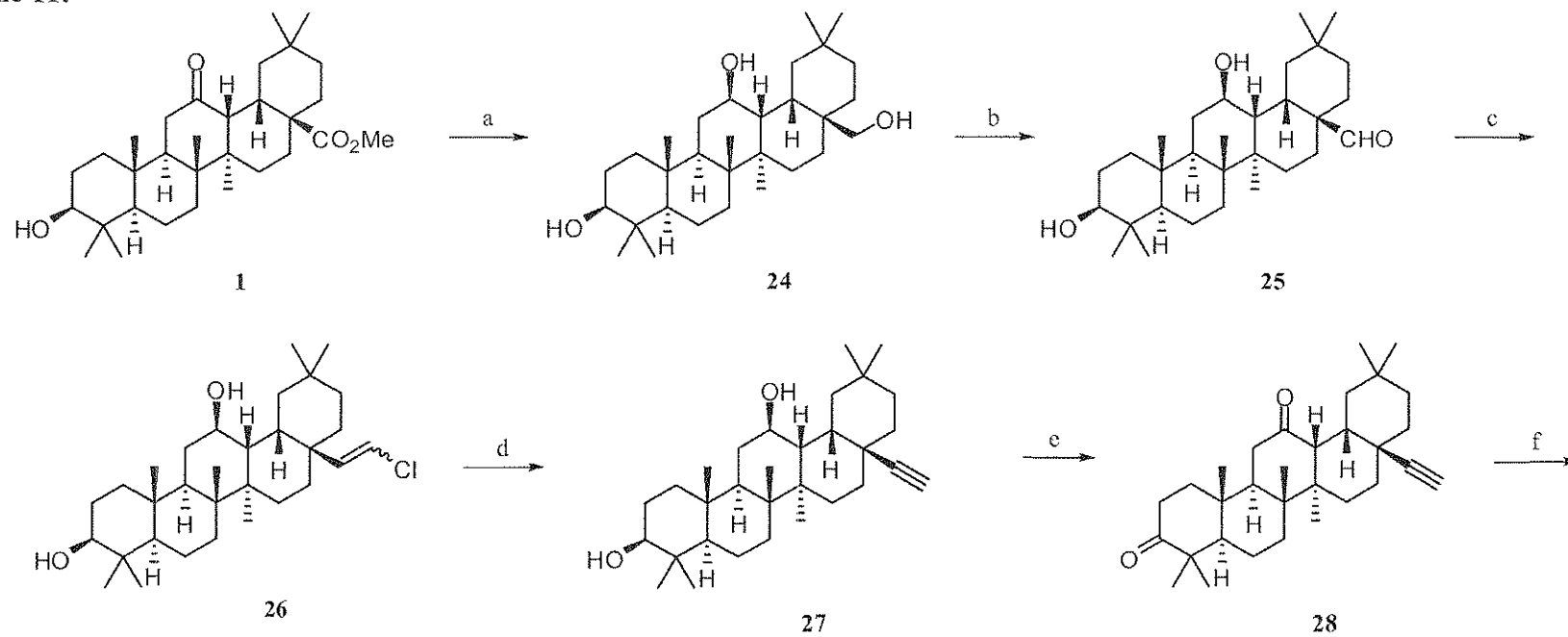
Scheme 11:
