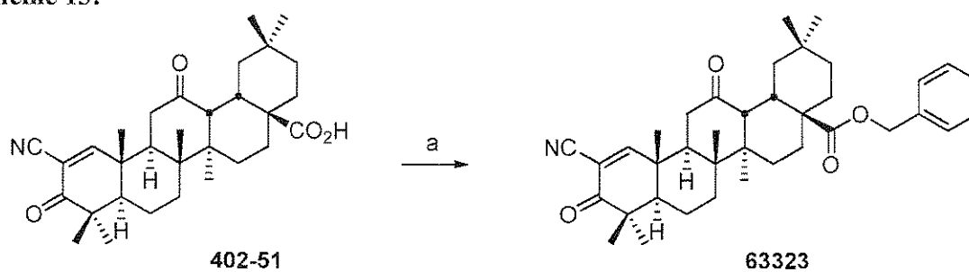
Scheme 13:
