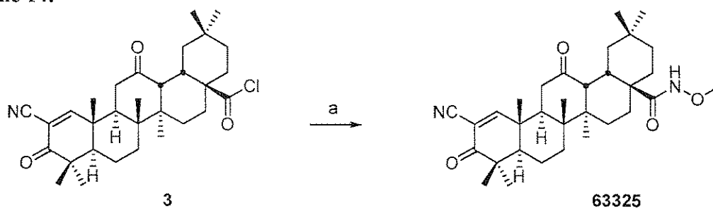
5 Scheme 14:
