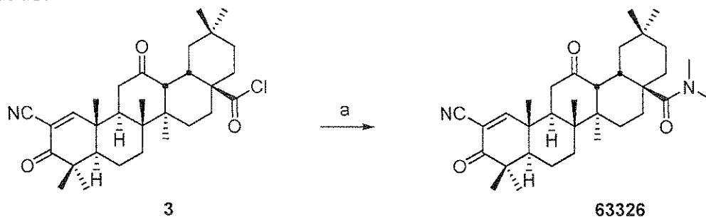
Scheme 15:
