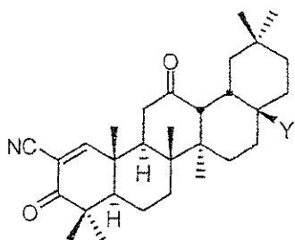
(XII),
