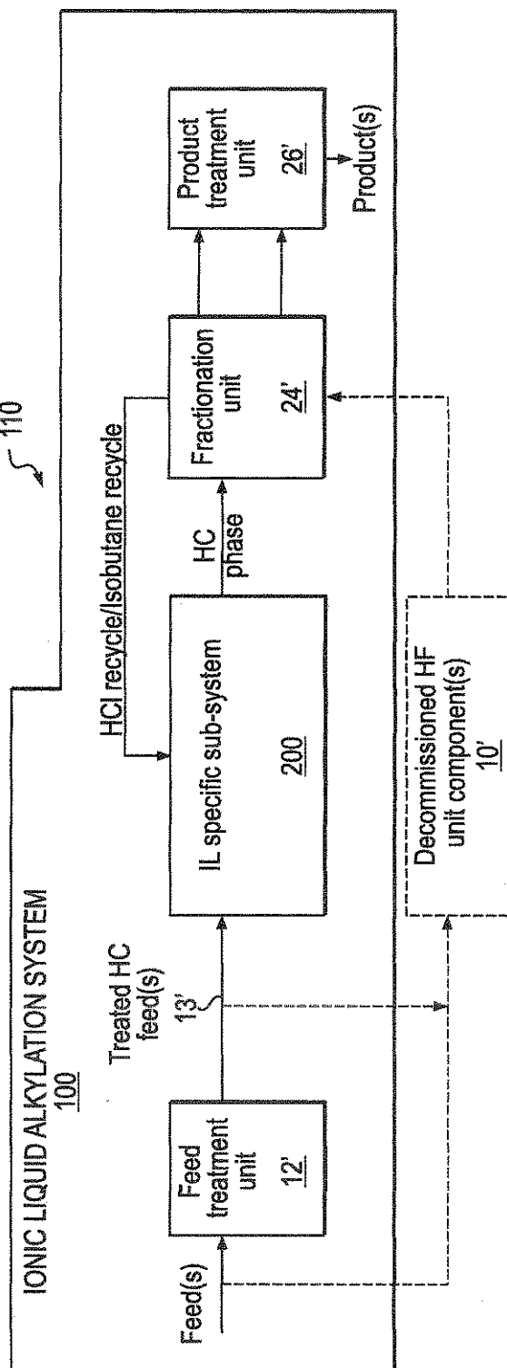
CONVERTED ALKYLATION SYSTEM 110
