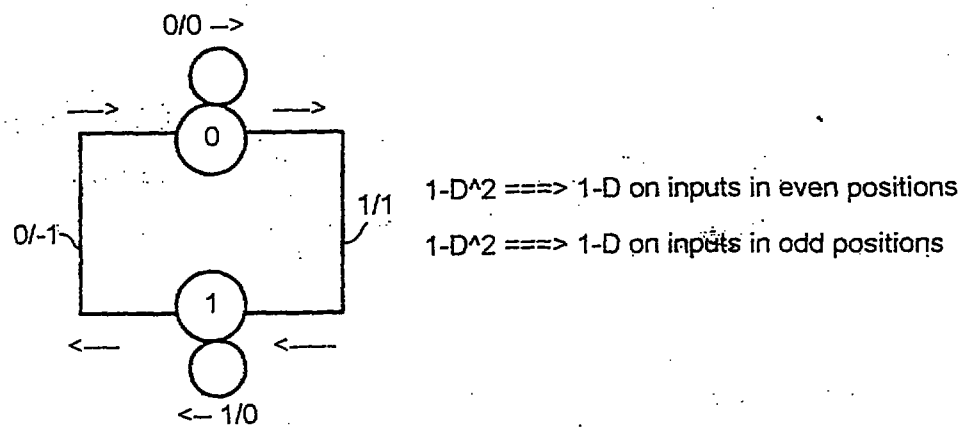
STATE DIAGRAM FOR c(i) = b(i) - b(i-1)
