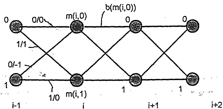
STATE DIAGRAM FOR c(i) = b(i) - b(i-1)
