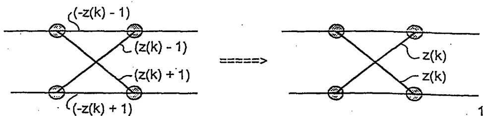
FIG. 8D TRELLIS TRANSFORM FOR PR4, MF CASE, \{+1, -1\} INPUTS
