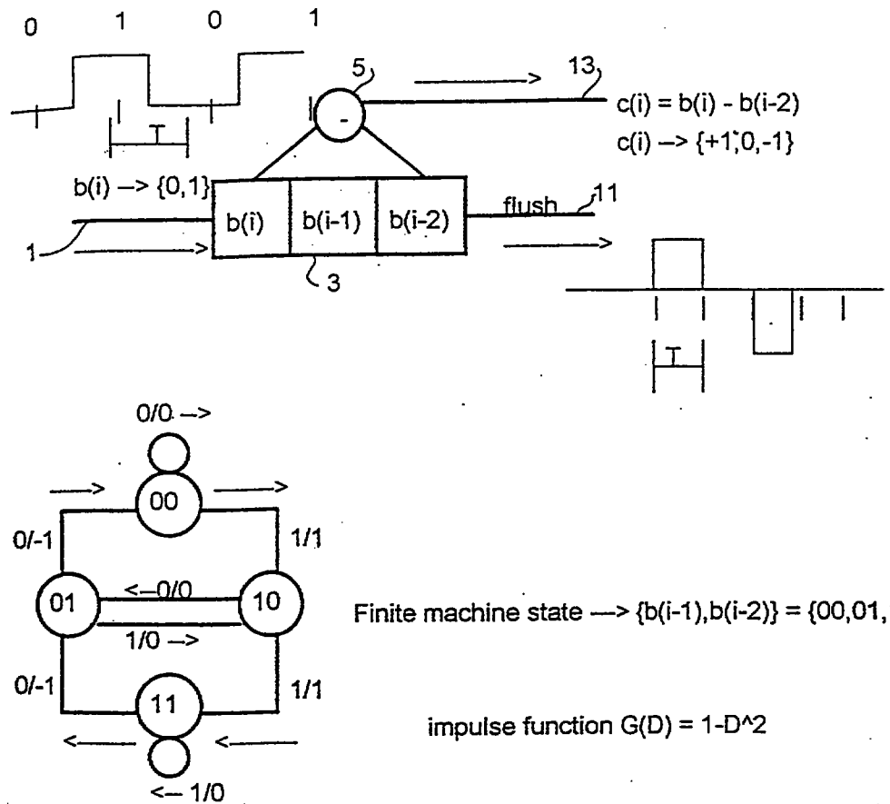
PARTIAL RESPONSE WAVEFORM ENCODER AND STATE DIAGRAM
