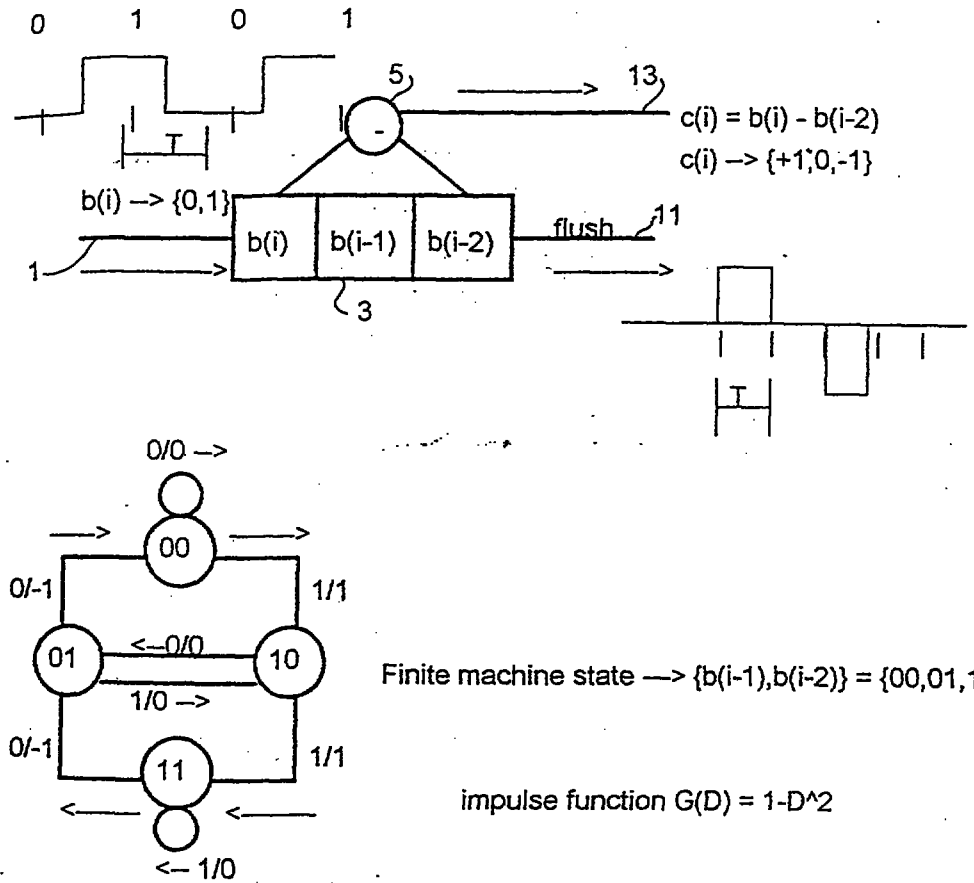
PARTIAL RESPONSE WAVEFORM ENCODER AND STATE DIAGRAM
