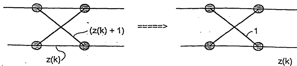
FIG. 8E TRELLIS TRANSFORM FOR PR4, MF CASE, \{0, 1\} INPUTS
