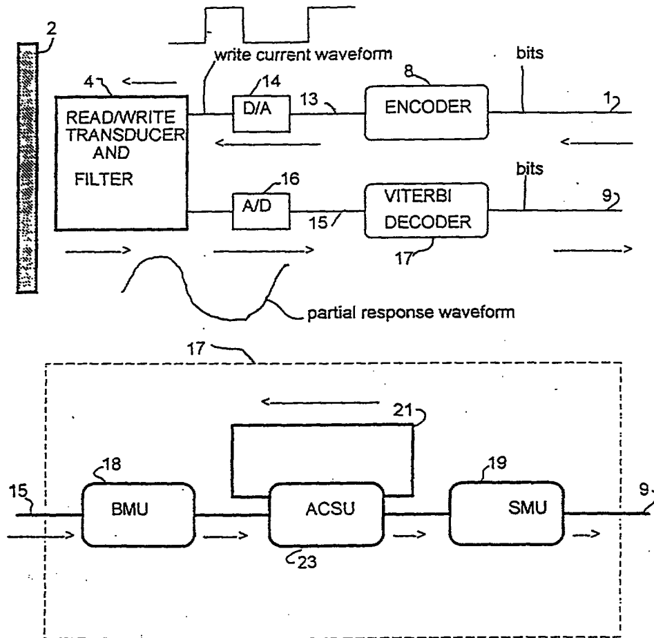
VITERBI DECODER AND ITS RECORDING CHANNEL SETTING
