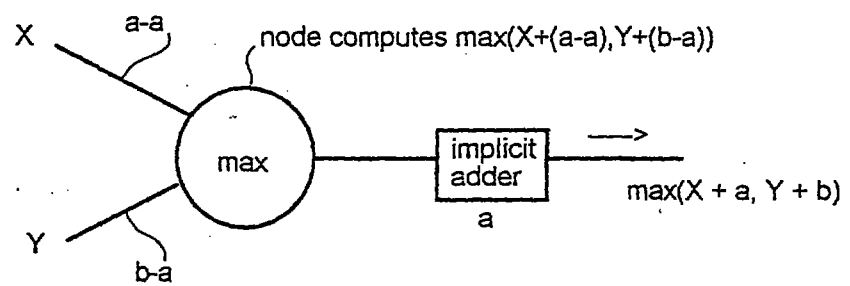
TRANSFORMED FLOW GRAPH
