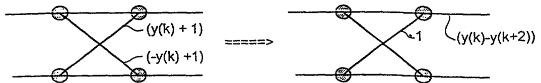
FIG. 8C TRELLIS TRANSFORM FOR PR4 WMF CASE
