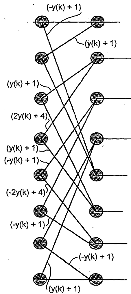
TRELLIS FOR EPR4, WMF CASE, {+1,-1} INPUTS
