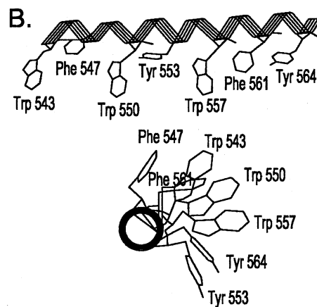
Butyrylcholinesterase Tetramer
