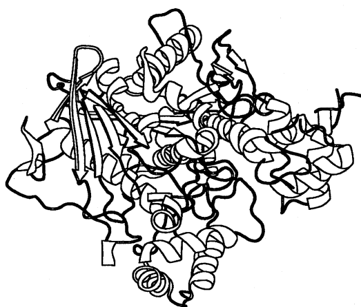
Butyrylcholinesterase Monomer
