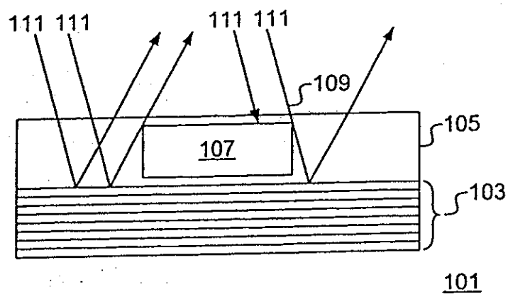
FIGURE 1 (PRIOR ART)
