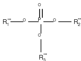
Formula IV
