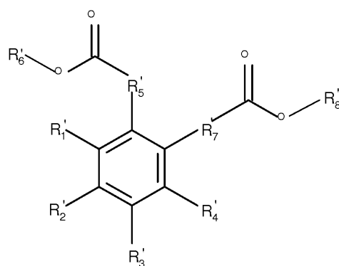
Formula II-(c)
