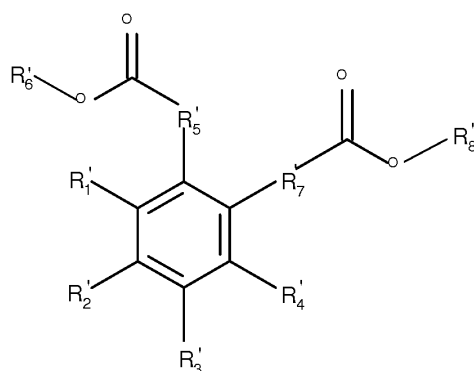
Formula II-(c)
