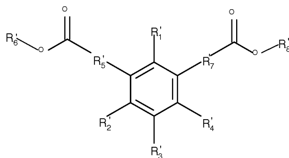
Formula II-(a)
