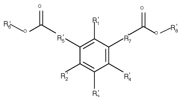
Formula II-(a)
