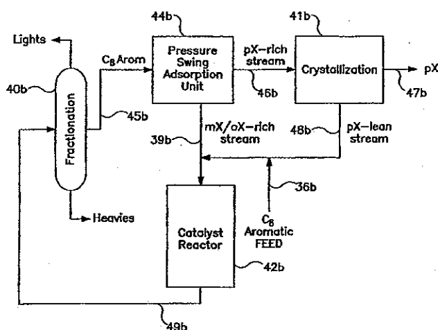
Embodiment 1: One Catalyst Reactor System
