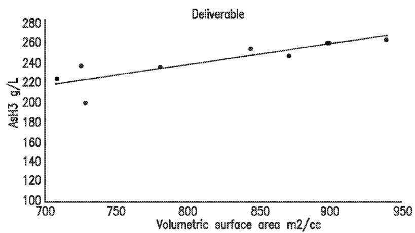
Arsine Deliverable Capacity versus Volumetric Surface Area for Structurally Modified Carbon Adsorbent Samples
