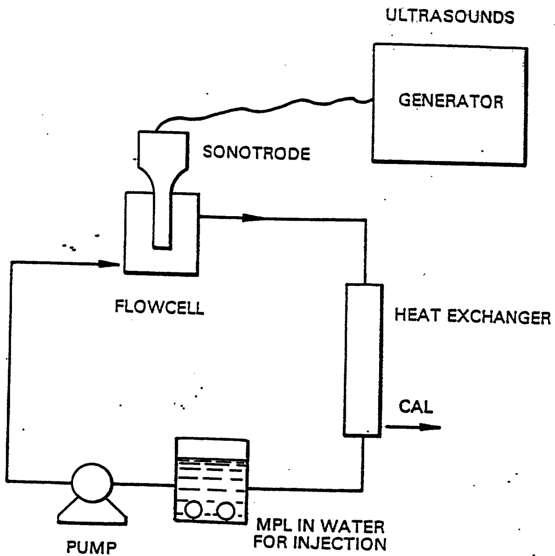
SONICATION LOOP
