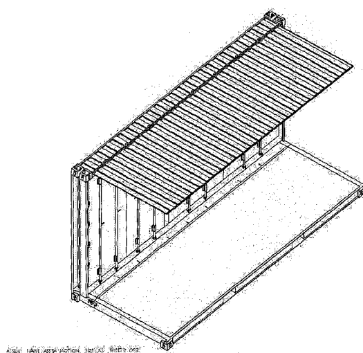
Figure 3 The folded state of the folding container after the first folding step.
