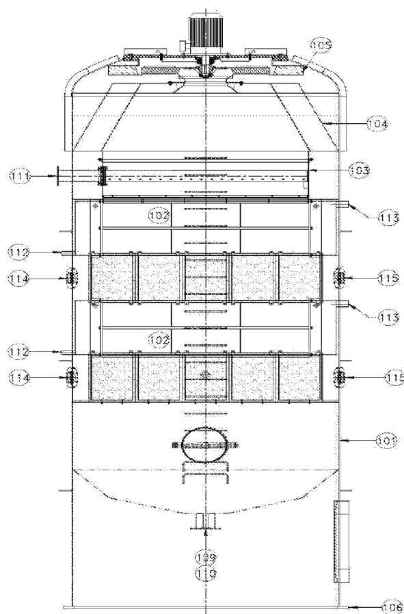
Fig. 2: Enlarge front view of vertical low temperature evaporator
