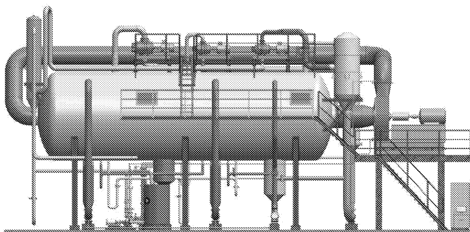
Fig. 11: 3D view of horizontal multi-effect low temperature evaporator
