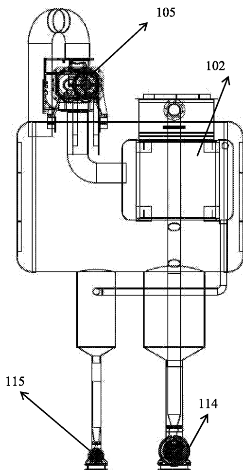
Fig. 7: Front view of horizontal single effect low temperature evaporator
