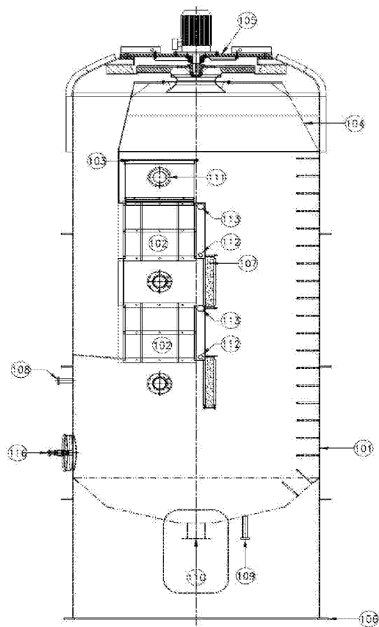
Fig. 1: Front view of vertical low temperature evaporator
