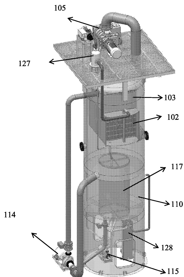
Fig. 4: 3D transparent view of vertical low temperature evaporator
