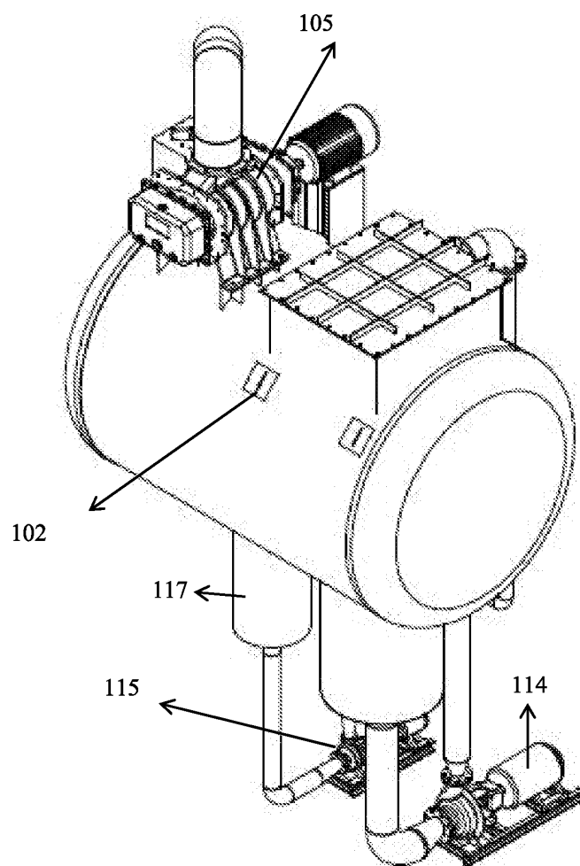
Fig. 6: Isometric view of horizontal single effect low temperature evaporator
