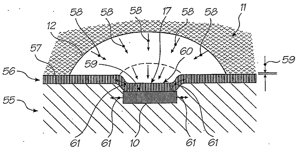
FIG. 47 (PRIOR ART)
