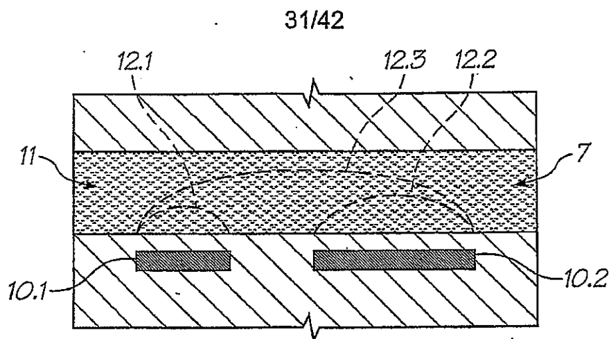
FIG. 52 (PRIOR ART)
