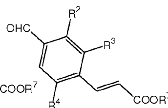
Structure 4
