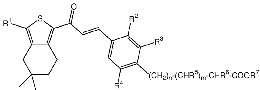
Formula (II)
