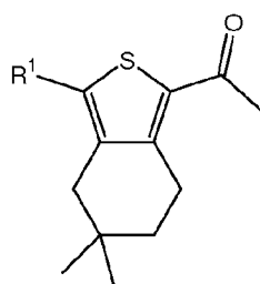
Structure 2
