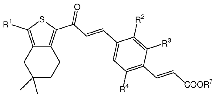
Formula (III)
