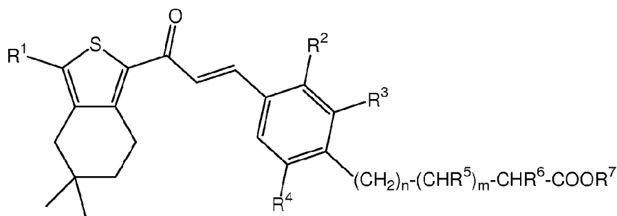
Formula (II)
