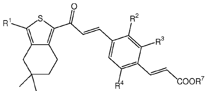
Formula (III)
