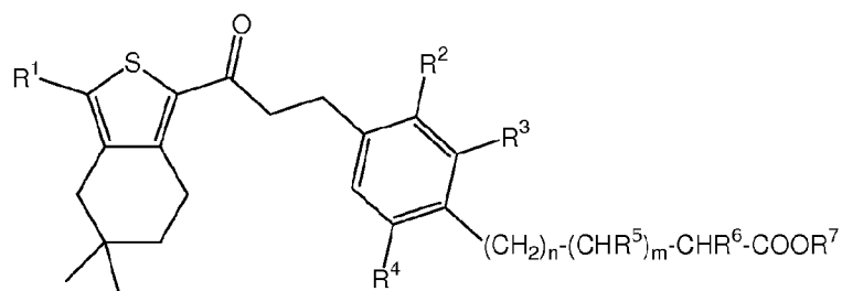
Structure 1
