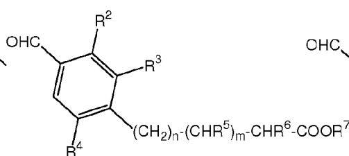
Structure 3
