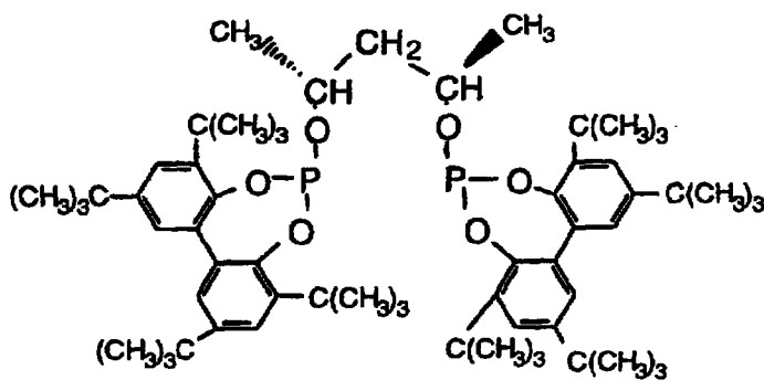
Ligand H
