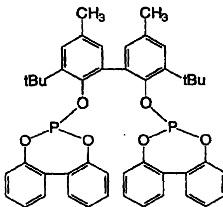
Ligand X
