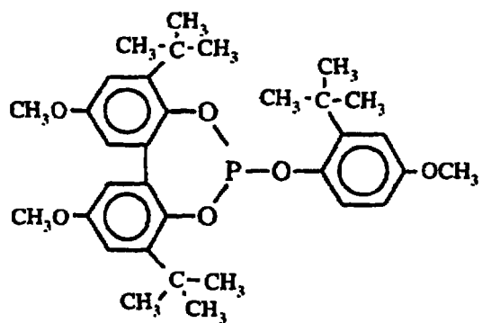
Ligand A
