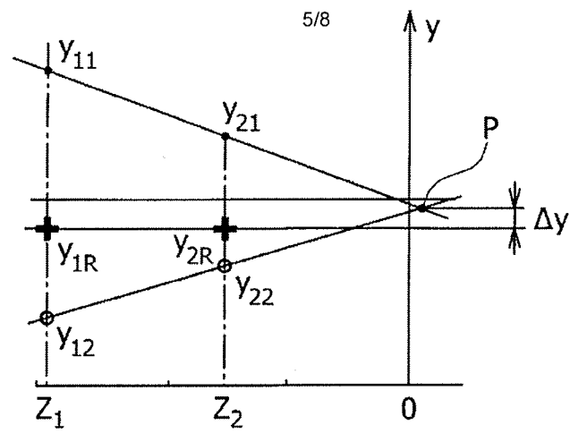
HEIGHTWISE POSITION Z OF TOOL TIP END PORTION
