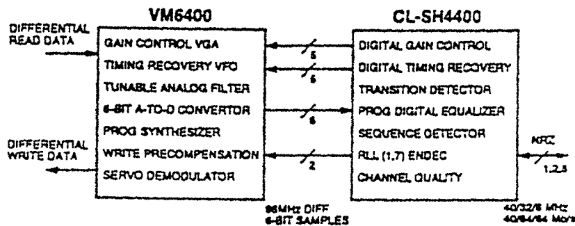
Figure 1 CL-SH4400/VM6400 Functional Partition
