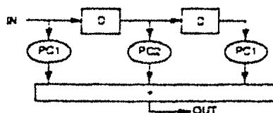
Figure 4.7-1 Pulse Shaping Filter Structure
