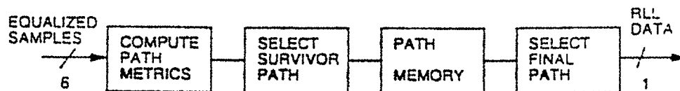
Figure 4.8-6 SoftTarget™ Sequence Detector
