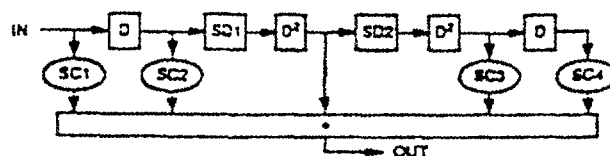
Figure 4.7-3 Spectrum Smoothing Filter Structure
