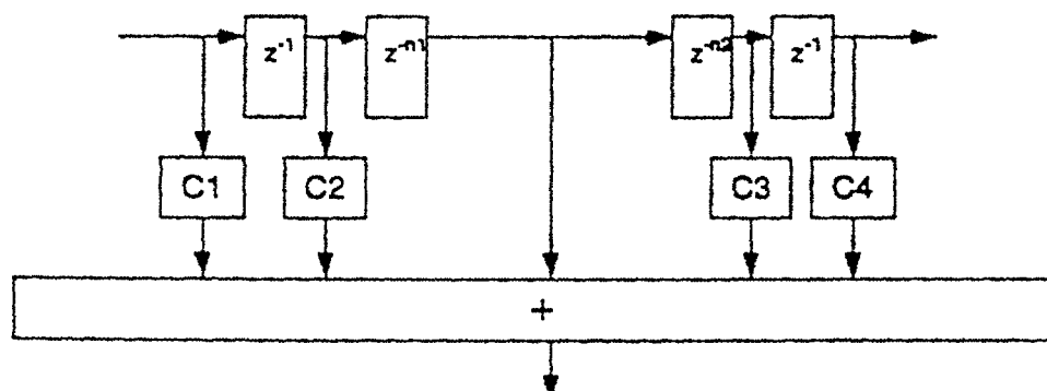
Figure 4.9.1 SFilter
