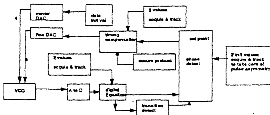
Figure 4.6.1 Timing Recovery Loop
