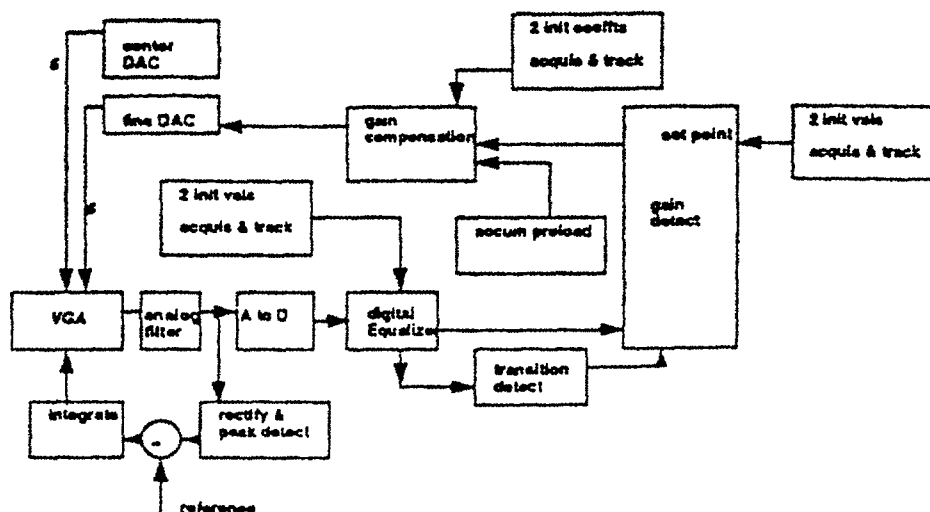
Figure 4.5.1. Gain Loop for data and servo
