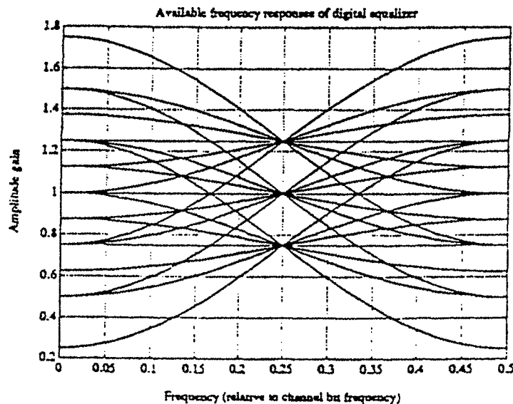
Figure 4.7-2 Pulse Shaping Filter Response
