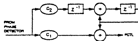
Figure 4.6-1 Timing Recovery Loop Compensation
