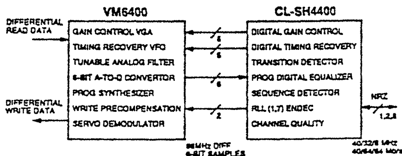
Figure 1 CL-SH4400/VM6400 Functional Partition
