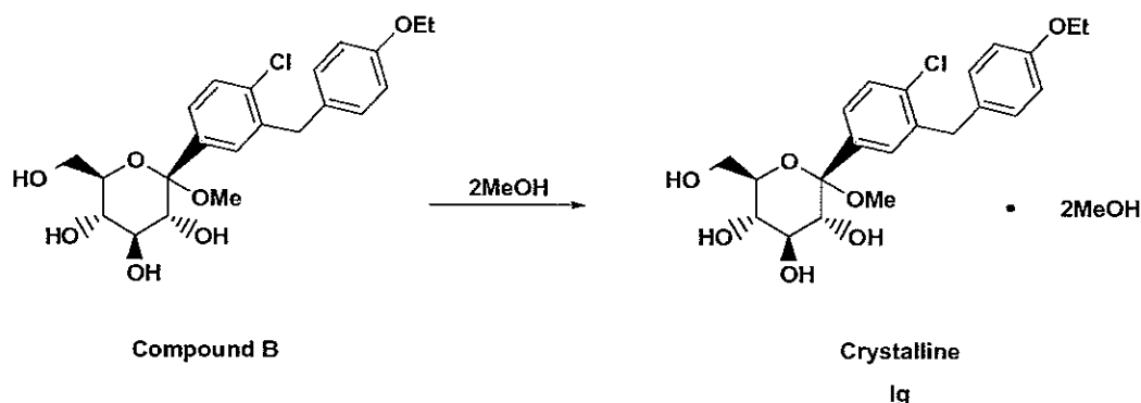
SCHEME V
