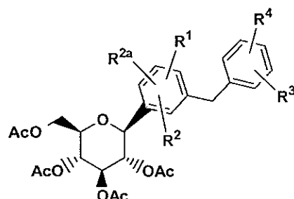
Compound C
