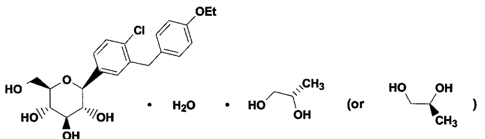
Compound Ia
