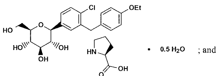
Compound Ij
