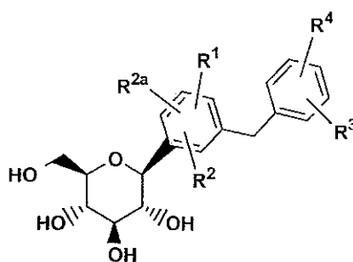
Compound D
