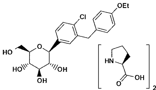
Compound Ih
