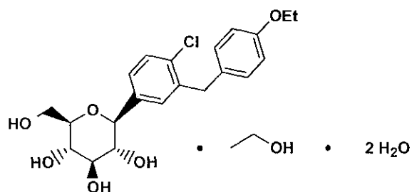
Compound Ic
