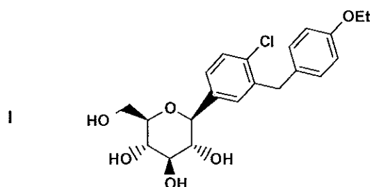
Compound I
