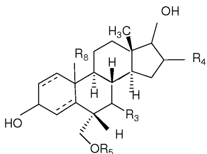
Formula (VIII)-A
