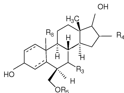
Formula (VIII)-B
