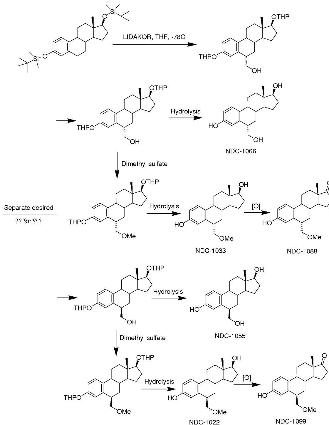
Scheme 1 - preparing compounds of the instant invention.
