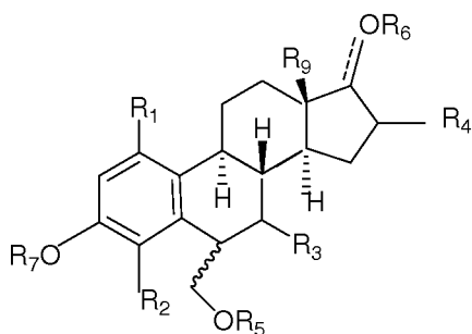
25 Formula (I)
