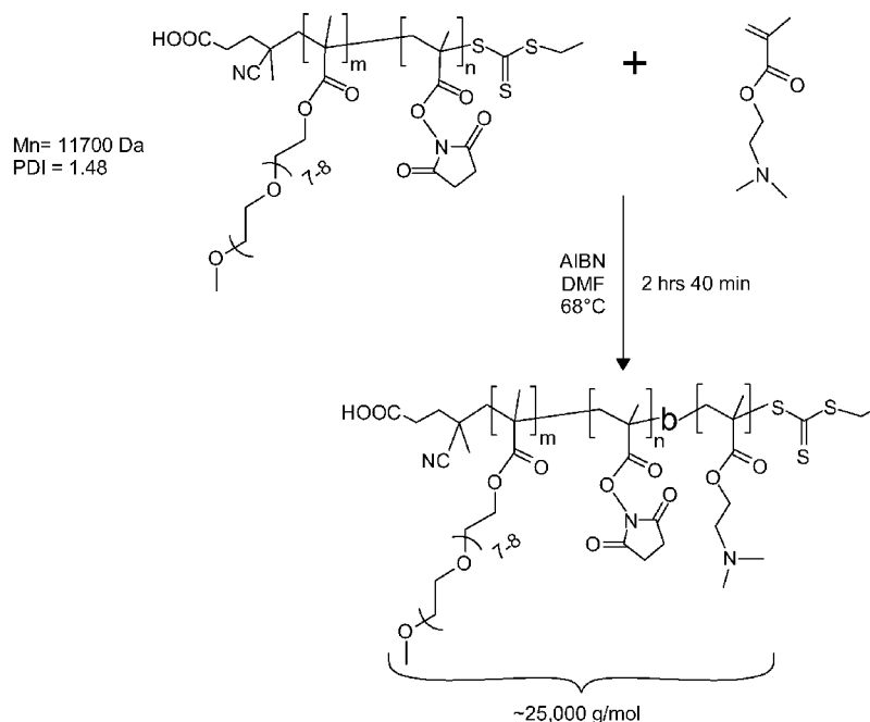
Fig. 1 Synthesis of poly(PEGMA-MANHS)-b-(DMAEMA)
