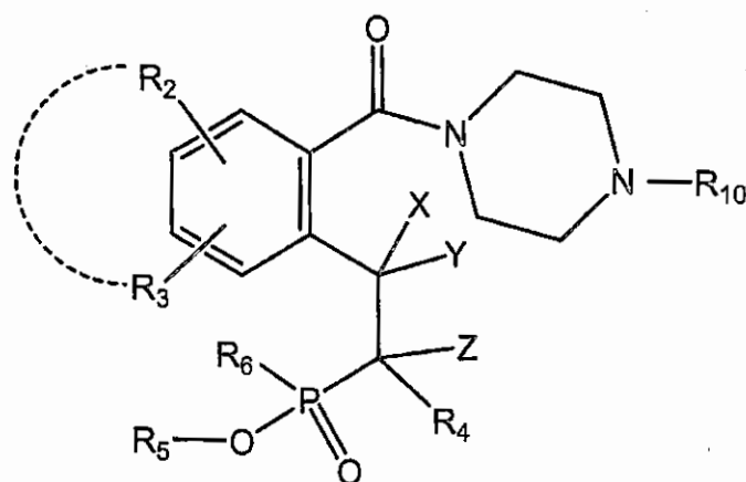
Formula (II)
