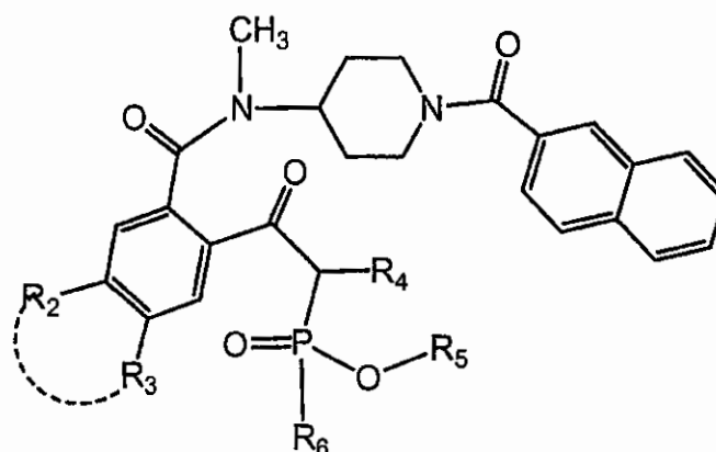
Formula (Ic)
