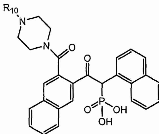
Formula IIa
