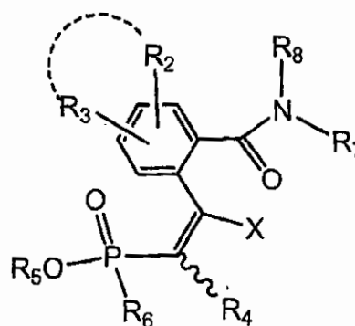
Formula (E)
