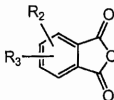
Formula (F)
