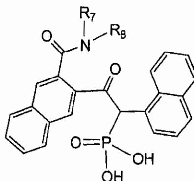
Formula (Ia)
