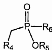
Formula (G)
