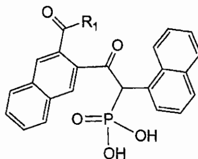
Formula (Ib)
