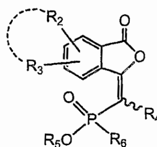
Formula (C)
