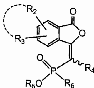
Formula (C)
