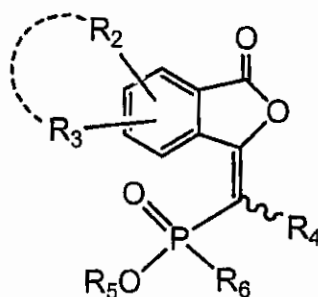
Formula (C)
