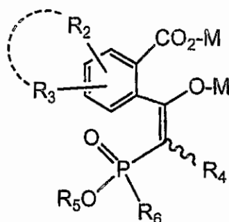
Formula (H)
