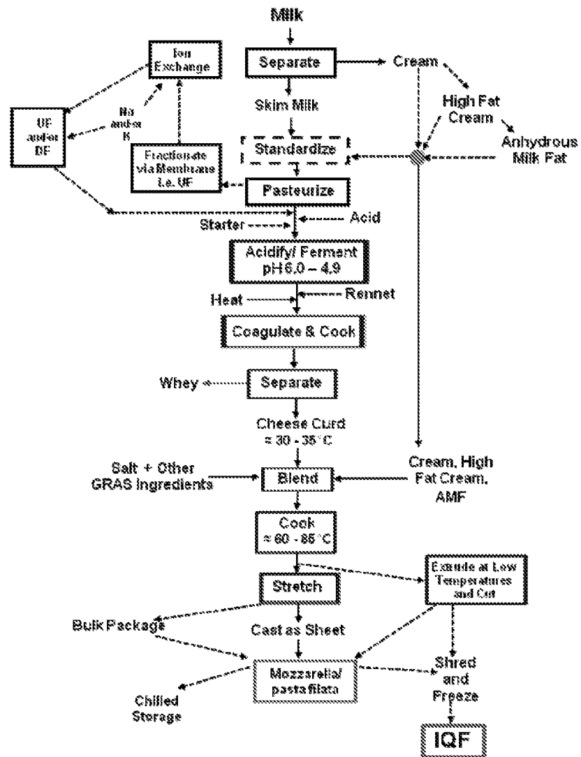
Figure 1: Fonterra Mozzarella manufacturing process
