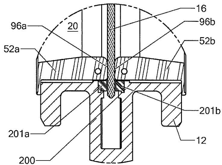
DETAIL K
