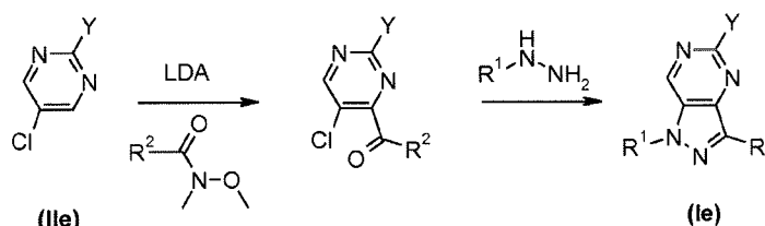
Scheme 5. General synthetic route for preparation of compounds of formula (Ie).
