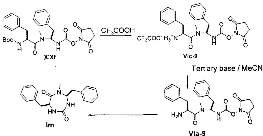
Diagram 11: Preparation of the compound (Im).
