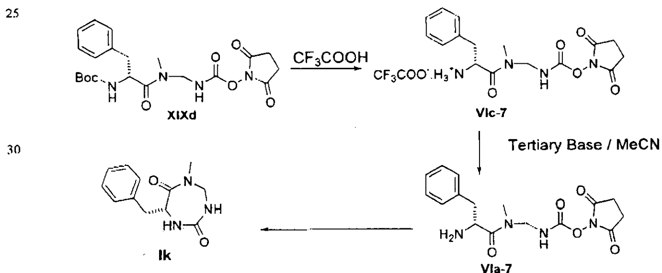
Diagram 9: Preparation of the compound (Ik).
