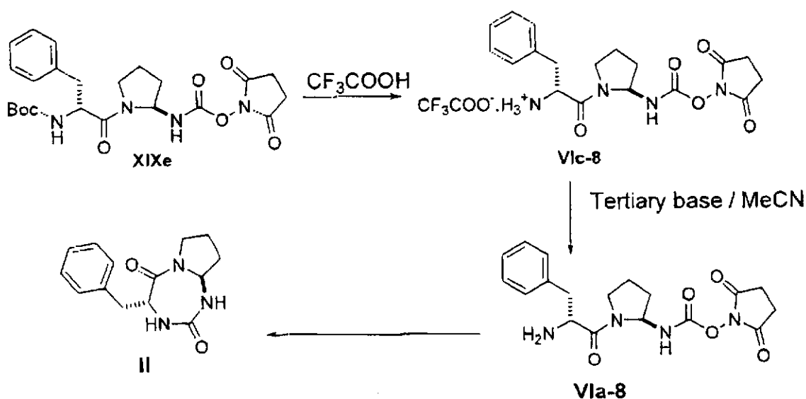
Diagram 10: Preparation of the compound (II).
