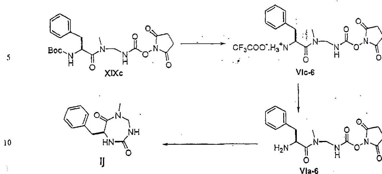
Diagram 8: Preparation of the compound (Ij).
