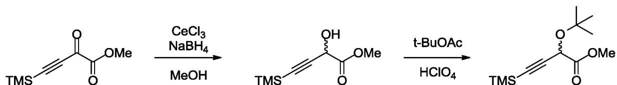
rac -Methyl 2-( tert -butoxy)-4-(trimethylsilyl)but-3-ynoate
