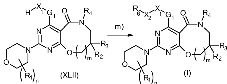
Scheme 1: reaction scheme for preparing the compound of formula (I) from the compound of formula (XLII).
