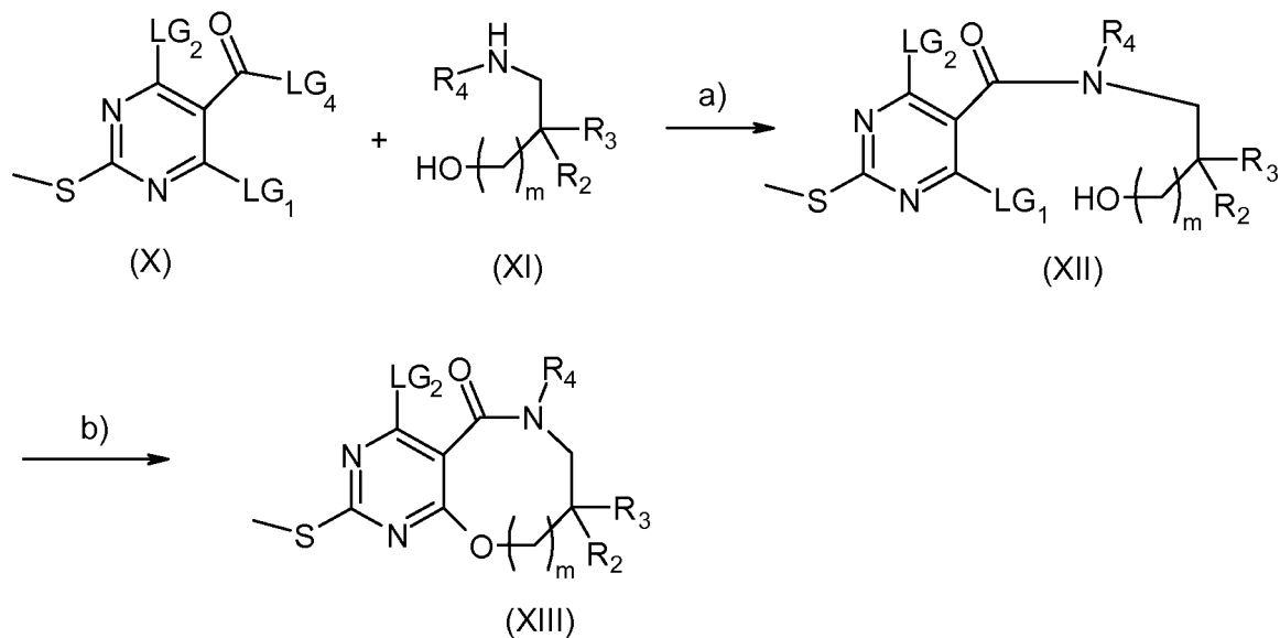
Scheme 5: reaction scheme for the preparation of the compound of formula (XIII) starting with the compound of formula (X) via steps a) and b).
