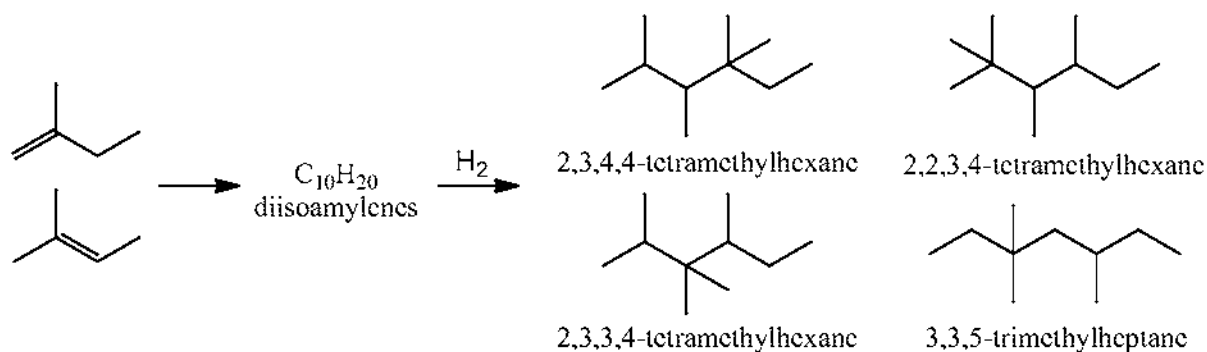
Scheme XIV
