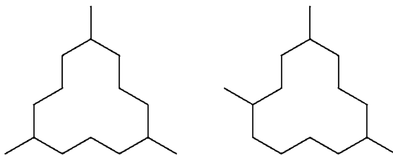
1,5,9- and 1,5,10-trimethylcyclododecane from cyclic trimerization of isoprene
