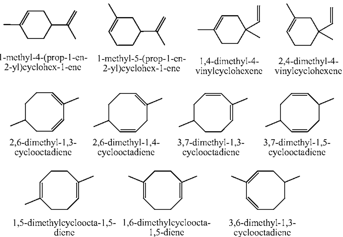
Scheme I. Exemplary unsaturated 6- and 8-membered ring intermediates
