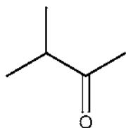
3-methyl-2-butanone
