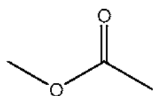
ethyl acetate
