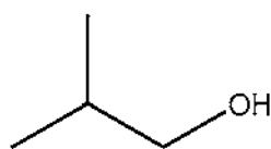
2-methyl-1-propanol
