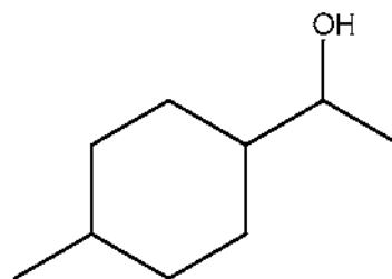
1-(1-hydroxyethyl)-4-methylcyclohexane
