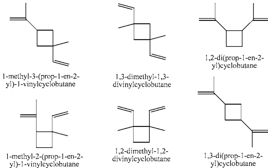
Scheme II. Exemplary unsaturated 4-membered ring intermediates
