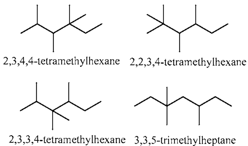
Scheme VIIIa. Examples of isodecanes derived from isoamylenes
