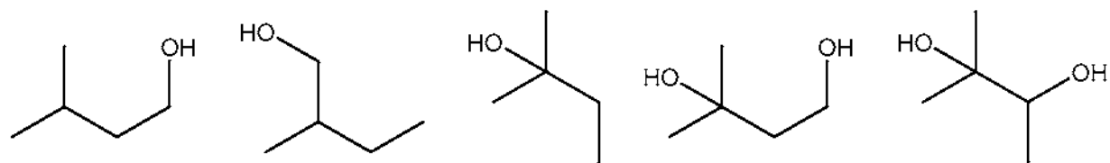
C5 alcohols and diols
