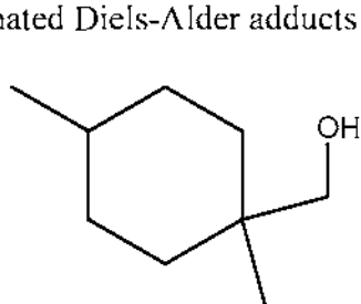
1,4-dimethyl-1-(hydroxymethyl)cyclohexane
