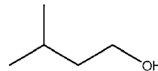
3-methyl-1-butanol
