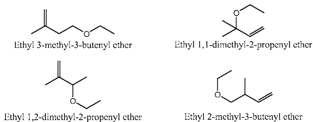
Scheme IV. Exemplary unsaturated ethyl ether intermediates
