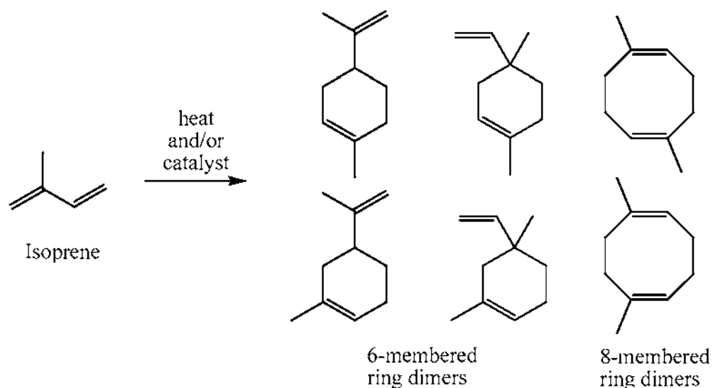
Scheme XI
