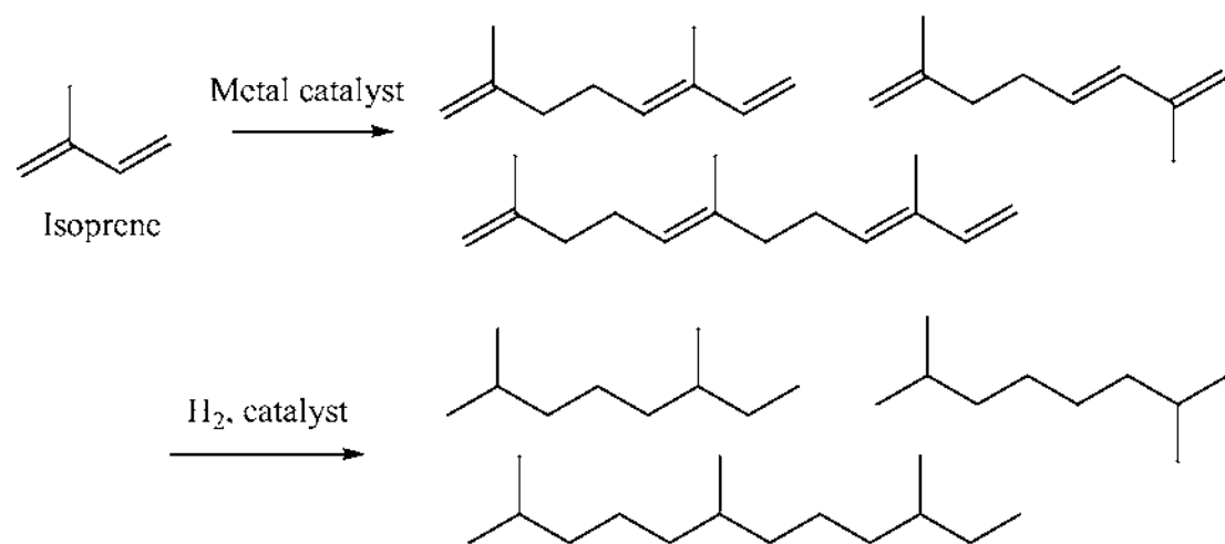
Scheme XII
