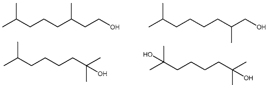
C10 alcohols and diols
