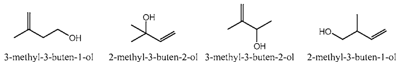
Scheme V. Exemplary unsaturated alcohol intermediates
