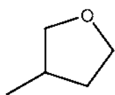
3-methyltetrahydrofuran
