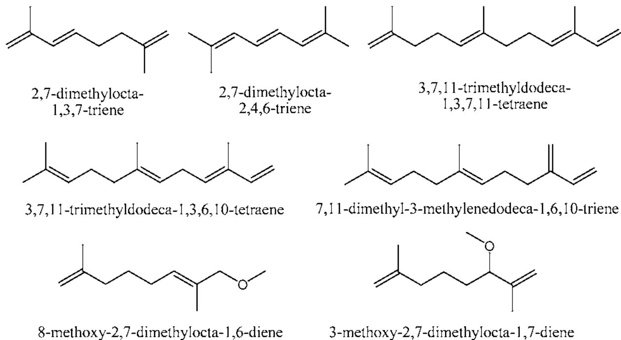
Scheme III. Exemplary unsaturated isoprene telomer and oxygenate intermediates
