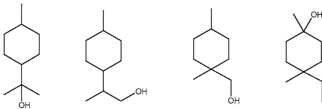
Cyclic C10 alcohols
