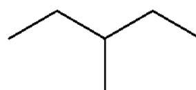
3-methylpentane
