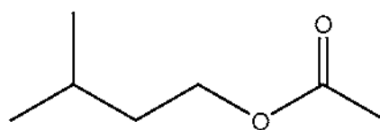
3-methyl-1-butyl acetate
