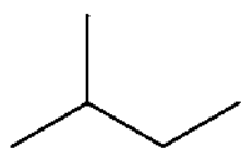
2-methylbutane
