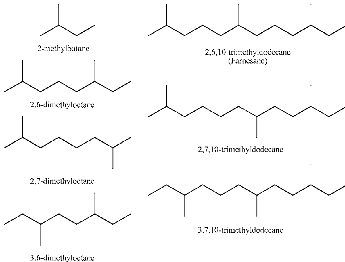
Scheme VIII. Examples of aliphatic hydrocarbons derived from isoprene
